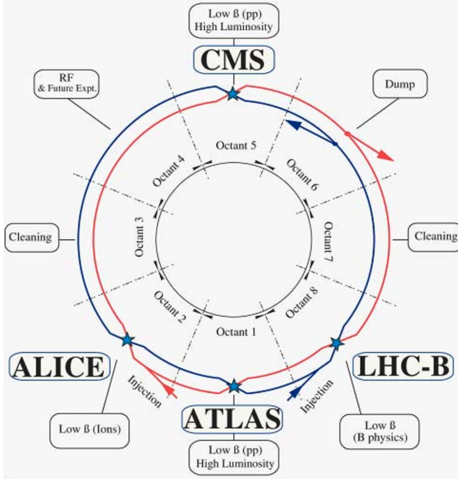
Figure 2.1. A simplified schematic of the overall layout of the LHC. The counter-rotating beams are shown in red (clockwise) and blue (counterclockwise). Reproduced from [19].
