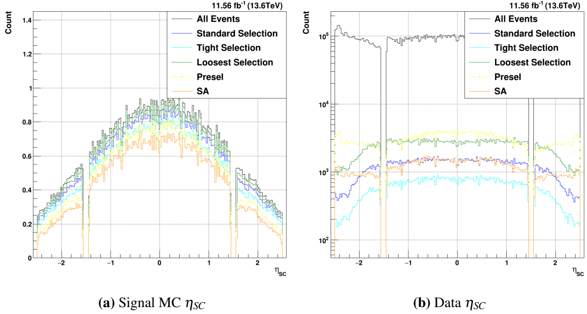
Figure 7.11. Total offline selection acceptances for HH \rightarrow b\bar{b}\gamma\gamma . Three tightnesses of BDT-based selection cuts are shown in dark blue (standard), light blue (tighter), and light green (looser). The acceptance of the preselection is shown in yellow, while the full standard analysis cuts are shown in orange. Both the lead and sublead photons are plotted together.
