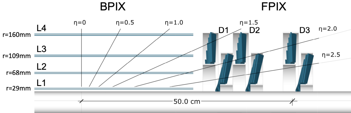
Figure 2.3. Longitudinal view of the pixel detector, where the beampipe is represented at the bottom of the image. Reproduced from [6]
