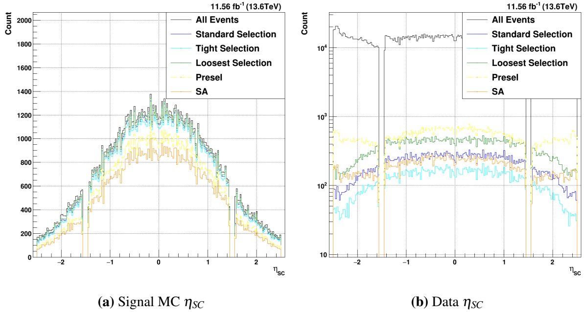
Figure 7.11. Both the lead and sublead photons are plotted together.
