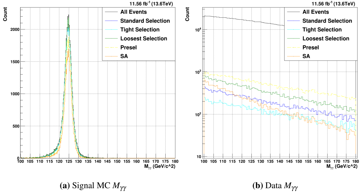
Figure 7.10. Both the lead and sublead photons are plotted together.
