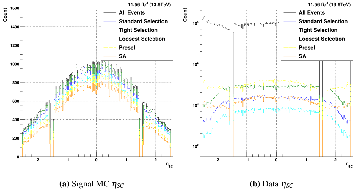
Figure 7.8. Both the lead and sublead photons are plotted together.
