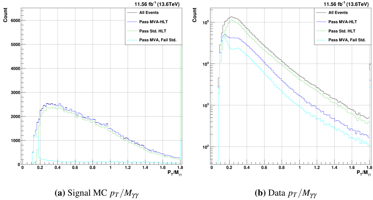
Figure 7.6. Acceptance of the MVA-HLT (blue) vs. the current standard diphoton HLT (green) for p_T/M_{\gamma\gamma}
