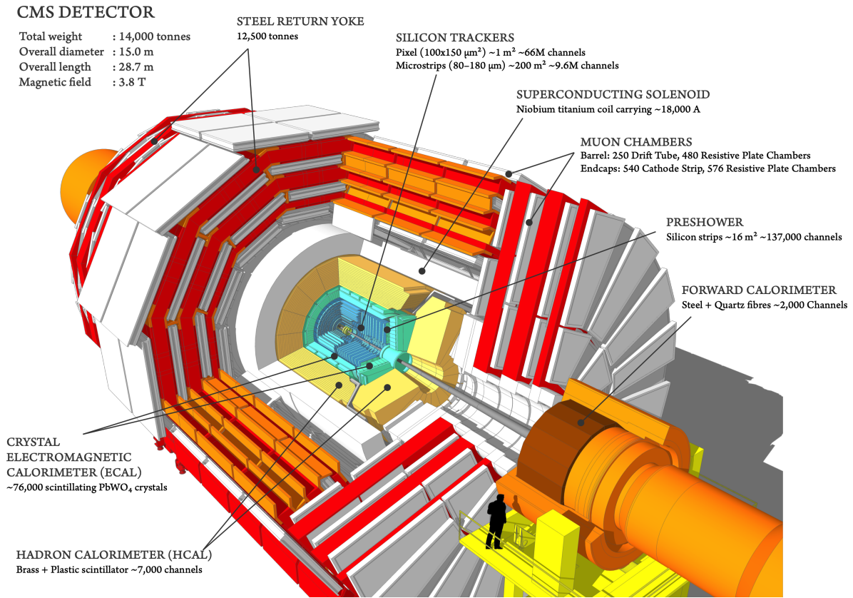
Figure 2.2. A full view of the CMS Detector, with each major system labeled. Reproduced from [7].
