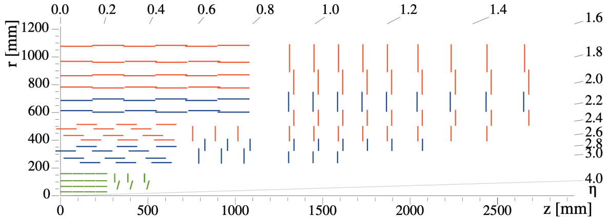
Figure 2.4. Full view of the tracker system. The inner pixel tracker is shown in green. Reproduced from [7]
