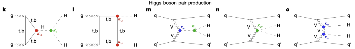
Figure 1.6. Feynman diagrams of known DiHiggs production modes. Figures k and l correspond to the two methods of ggH production, and m, n, and o correspond to the three methods of VBF production. Reproduced from [6].
