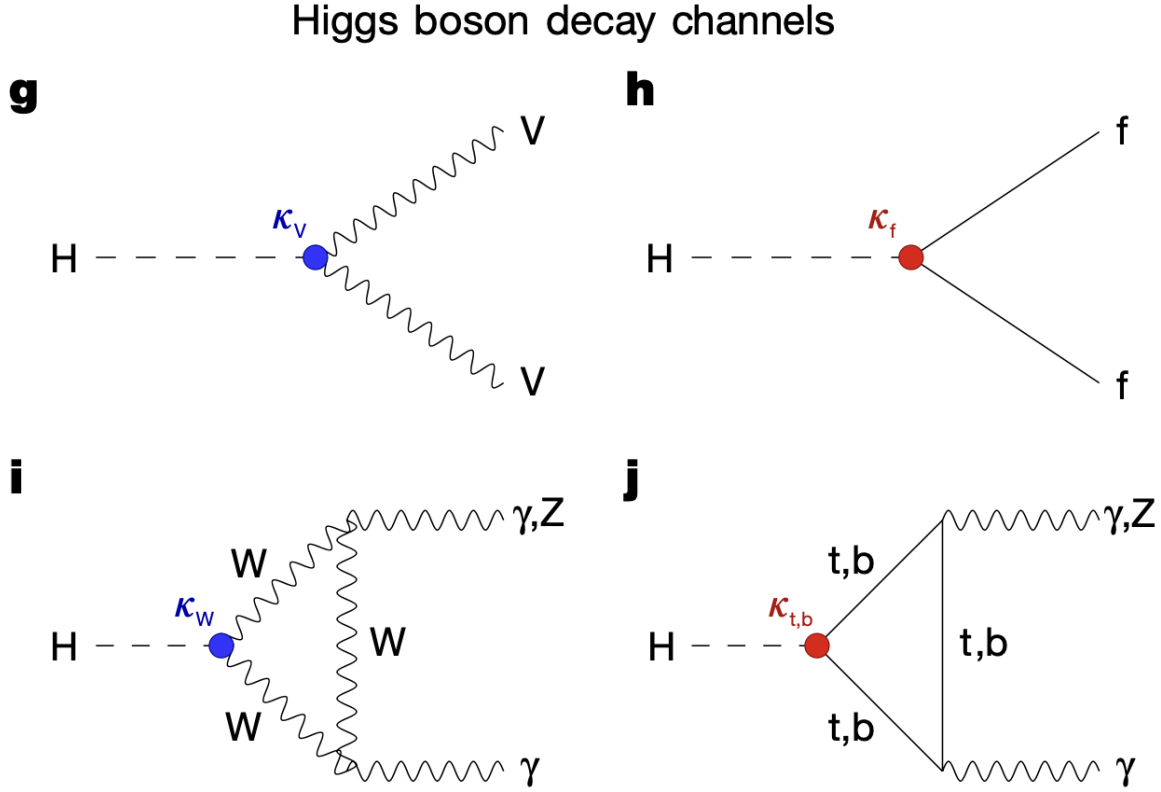
Figure 1.4. Feynman diagrams of known Higgs decay modes. Heavy vector bosonic decays are shown in g, fermion-antifermion decays are shown in h, and photon/Z boson decays are shown in i and j. Reproduced from [6]
