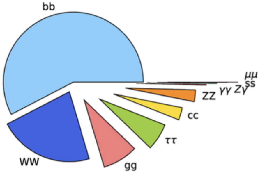
Figure 1.5. Theoretical branching fractions for a single Higgs. Reproduced from [6]
