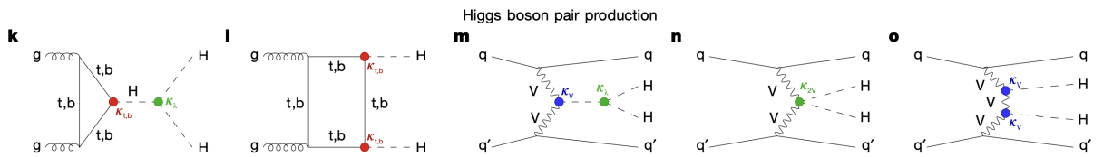
Figure 1.6. Feynman diagrams of known DiHiggs production modes. Figures k and l correspond to the two methods of ggH production, and m,n, and o correspond to the three methods of VBF production. Reproduced from [6].
