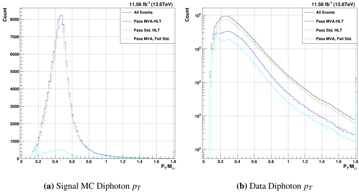
Figure 7.3. H \rightarrow \gamma\gamma acceptance of the MVA-HLT (dark blue) vs. the current standard diphoton HLT (green) for p_T . Both the lead and sublead photons are plotted together. Events that pass the MVA-HLT but fail the standard HLT can be seen in light blue.
