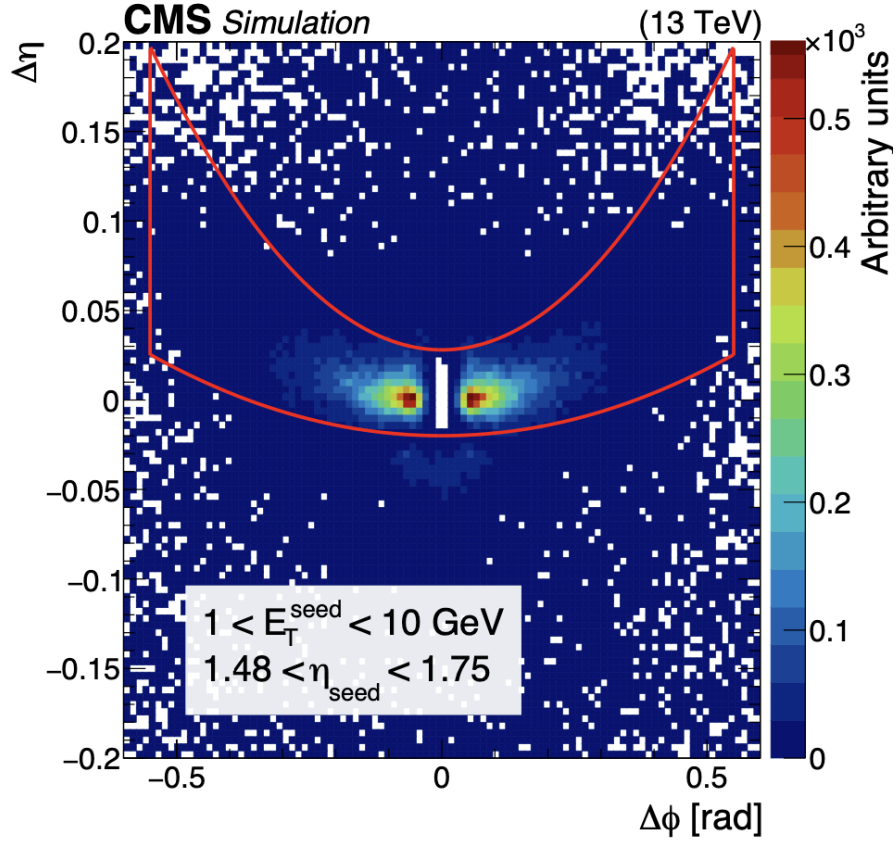
Figure 3.4. A distribution of the \Delta\eta versus \Delta\phi for the superclustering of simulated electrons. The color represents the number of clusters matched with the simulation around the seed. The red line represents the set of clusters selected by the mustache algorithm. The seed cluster can be seen as the white region in the center of the plot (where both \Delta\eta and \Delta\phi are equal to 0). The bending of the cluster due to the magnetic field can be seen in \phi , but not \eta . Reproduced from [24].
