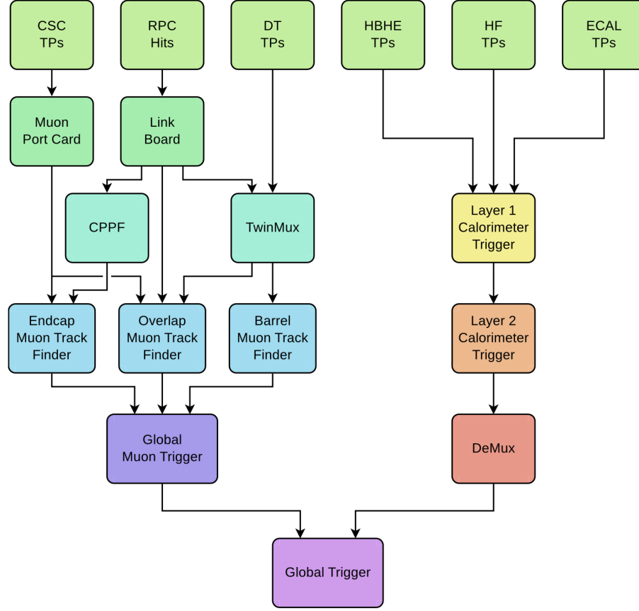
Figure 3.1. A diagram of the L1 Trigger architecture, where the lefthand tree corresponds to the muon triggers and the righthand tree to the calorimeter triggers. Reproduced from [21].
