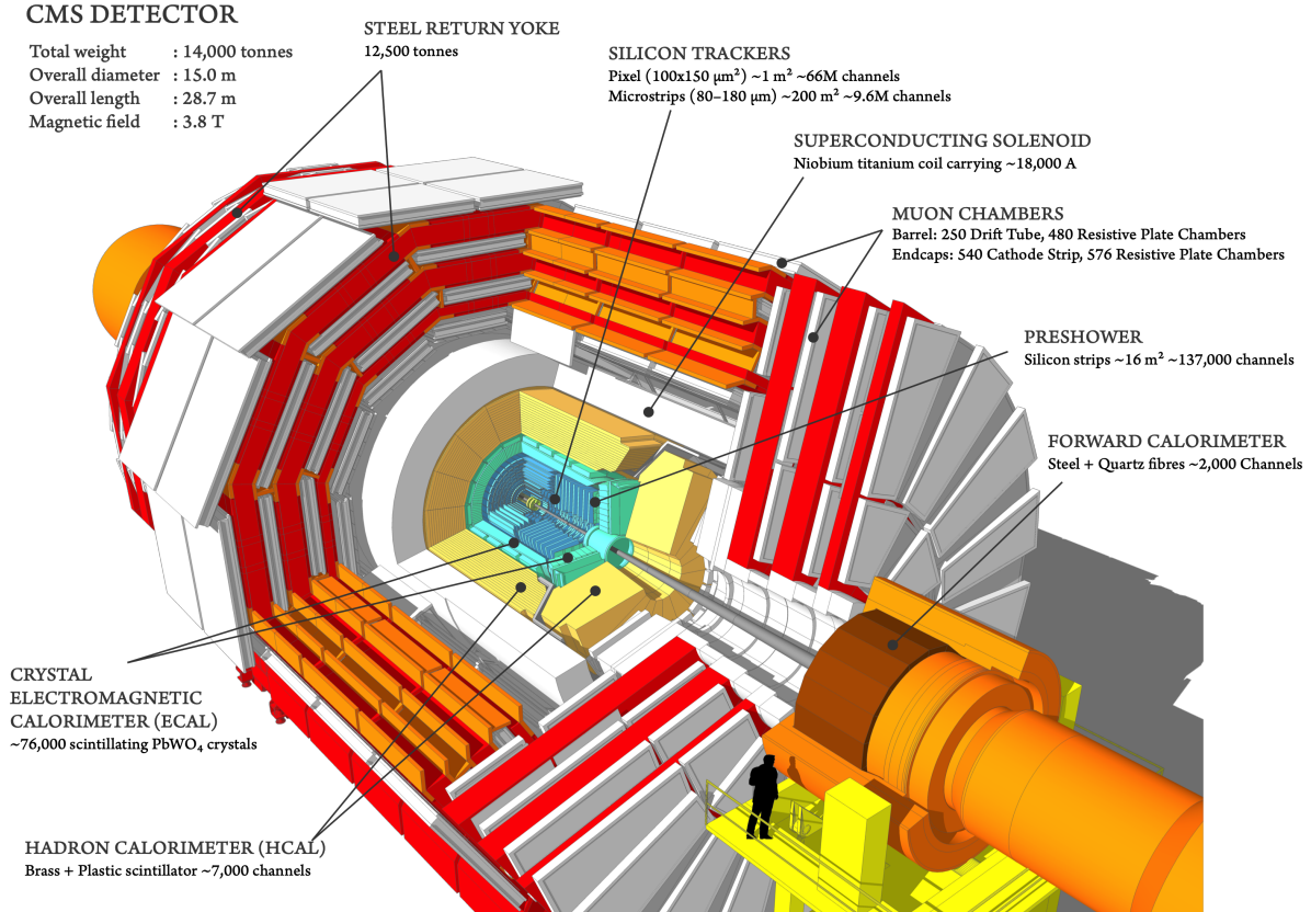
Figure 2.2. A full view of the CMS Detector, with each major system labeled. (Reproduced from [19])
