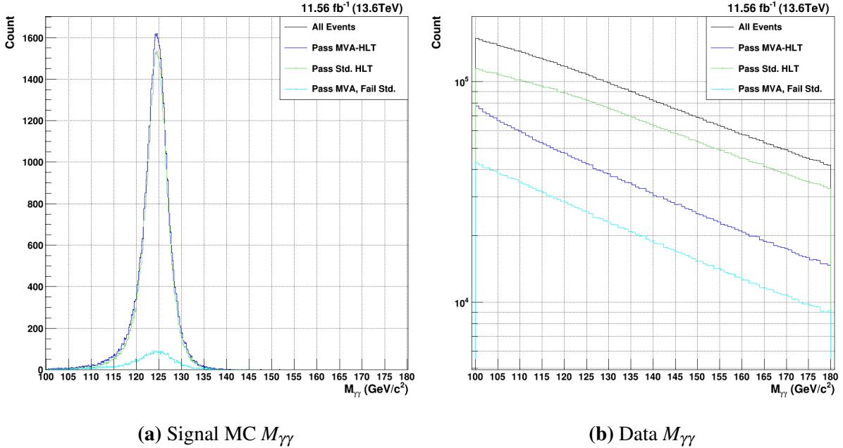
Figure 7.1. H \rightarrow \gamma\gamma acceptance of the MVA-HLT (dark blue) vs. the current diphoton sHLT (green) for M_{\gamma\gamma} . Events that pass the MVA-HLT but fail the sHLT can be seen in light blue.
