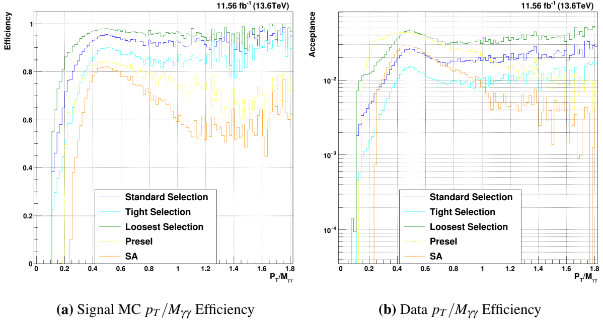
Figure 7.12. Total offline efficiency for H \rightarrow \gamma\gamma . Three tightnesses of BDT-based selection cuts are shown in dark blue (standard), light blue (tighter), and light green (looser). The acceptance of the preselection is shown in yellow, while the full standard analysis cuts are shown in orange.
