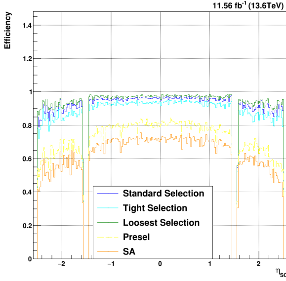
(a) Signal MC \eta_{SC} Efficiency
