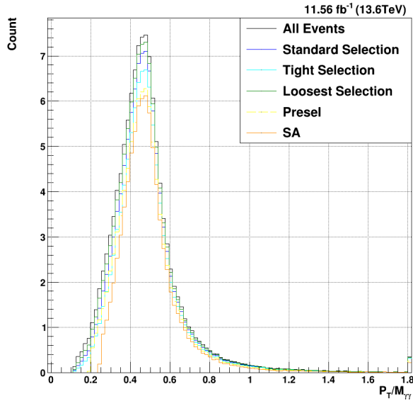
(a) Signal MC p_T/M_{\gamma\gamma}
