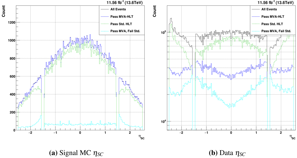
Figure 7.2. H \rightarrow \gamma\gamma acceptance of the MVA-HLT (dark blue) vs. the current diphoton sHLT (green) for \eta_{SC} . Both the lead and sublead photons are plotted together. Events that pass the MVA-HLT but fail the sHLT can be seen in light blue.
