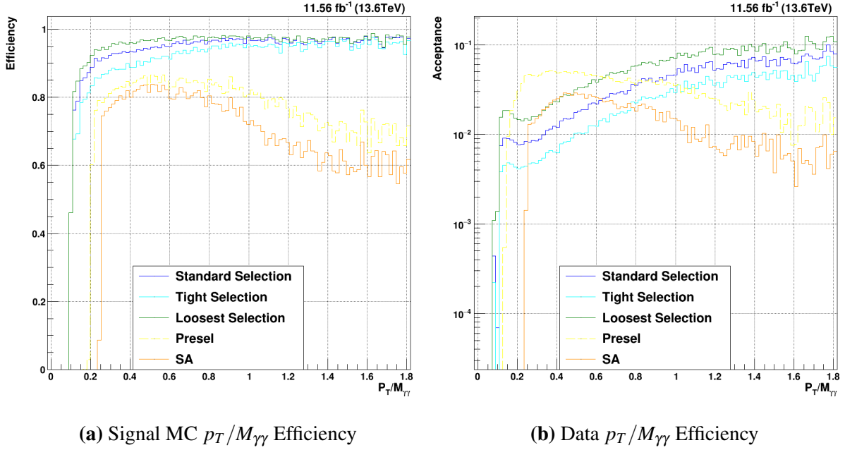
Figure 7.19. Total offline efficiency for HH \rightarrow b\bar{b}\gamma\gamma . Three tightnesses of BDT-based selection cuts are shown in dark blue (standard), light blue (tighter), and light green (looser). The acceptance of the preselection is shown in yellow, while the full standard analysis cuts are shown in orange.
