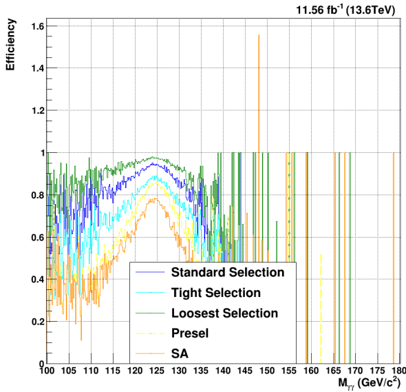
(a) Signal MC M_{\gamma\gamma} Efficiency
