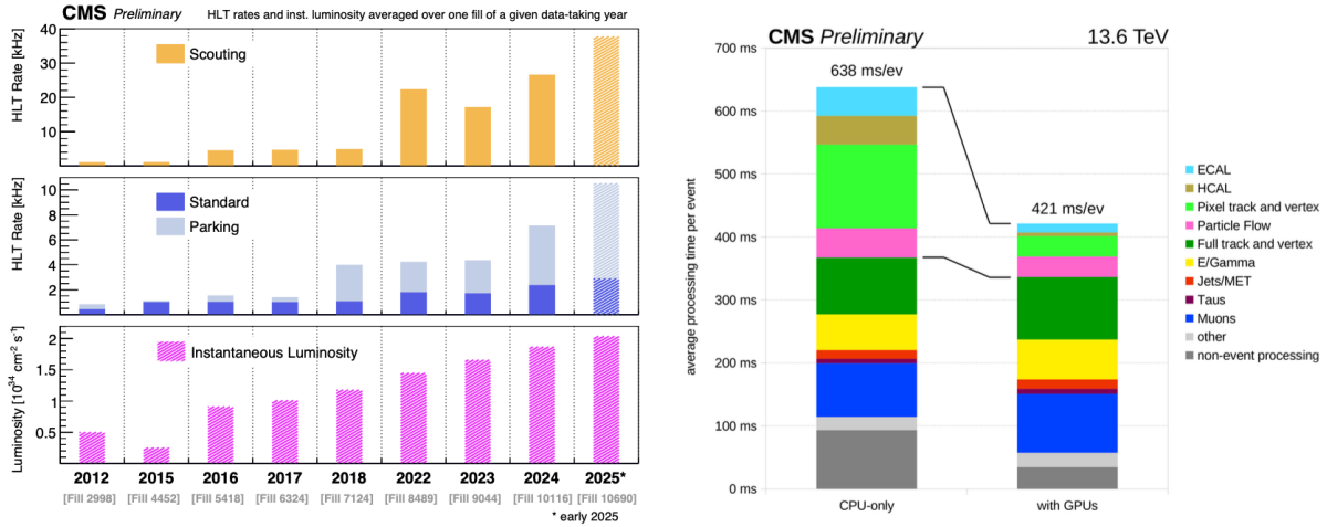
Figure 3.6. On the left, the rates of the scouting dataset (top), prompt (middle, solid), and parking (middle, hatched) data streams are shown. Additionally, the instantaneous luminosity is shown (bottom). To the right, the menu timing is shown with CPU-only and CPU+GPU processing for the 2022 running year. Reproduced from [17]
