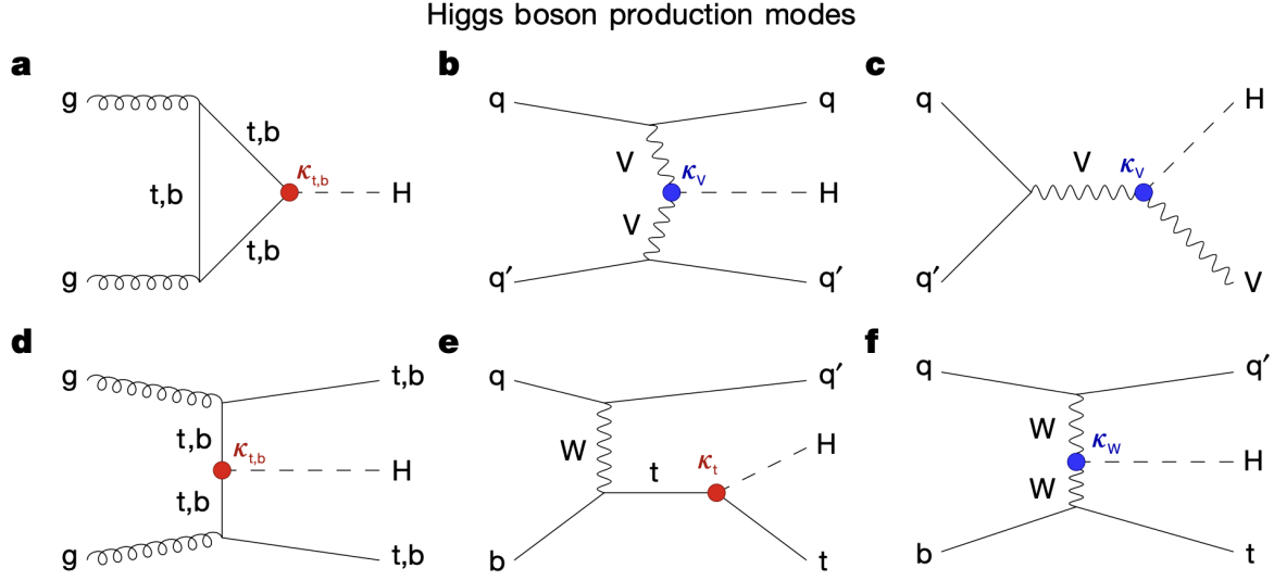
Figure 1.3. Feynman diagrams of known Higgs production modes. a is known as gluon fusion, termed ggH . b is known as vector boson fusion (VBF). c is production of the Higgs in association with a vector boson (either a W^\pm or Z^0 boson), called VH production. d is the production of the Higgs in association with a pair of top ( ttH ) or bottom ( bbH ) quarks. e and f both show Higgs production in association with a single top quark ( tH ). Reproduced from [13]
