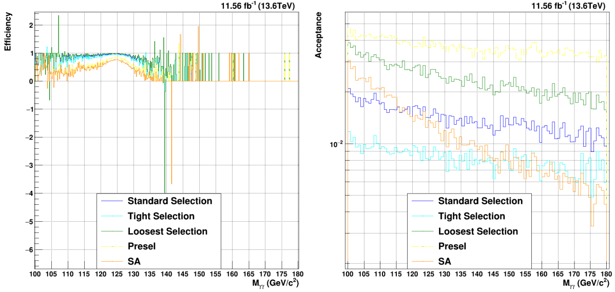
(a) Signal MC M_{\gamma\gamma} Efficiency
