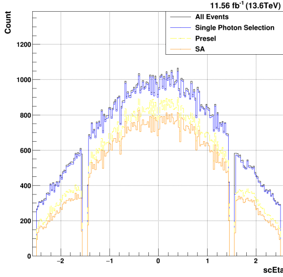
(a) Signal MC \eta_{SC}
