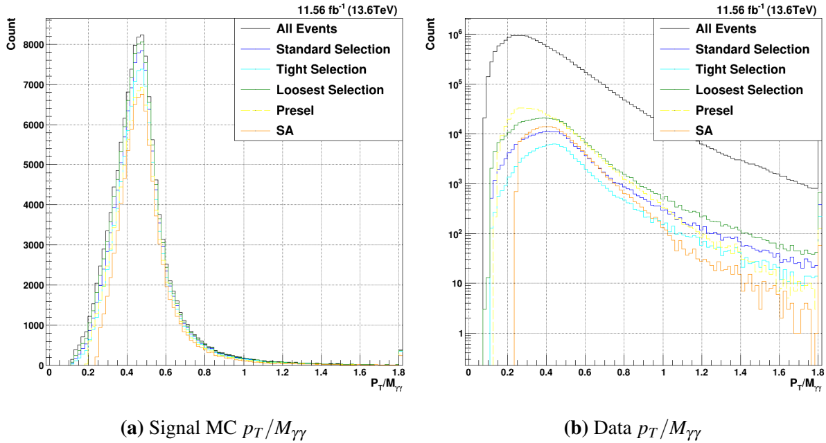
Figure 7.11. Total offline selection acceptances for H \rightarrow \gamma\gamma . Three tightnesses of BDT-based selection cuts are shown in dark blue (standard), light blue (tighter), and light green (looser). The acceptance of the preselection is shown in yellow, while the full standard analysis cuts are shown in orange. Both the lead and sublead photons are plotted together.
