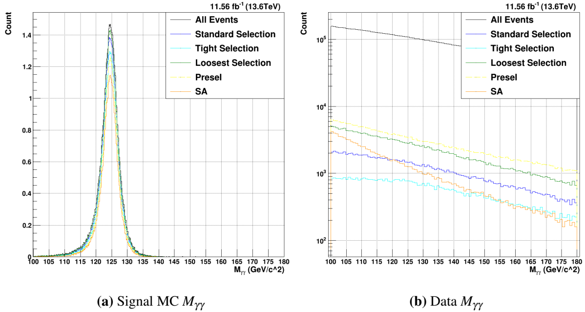
Figure 7.14. Total offline selection acceptances for HH \rightarrow b\bar{b}\gamma\gamma . Three tightnesses of BDT-based selection cuts are shown in dark blue (standard), light blue (tighter), and light green (looser). The acceptance of the preselection is shown in yellow, while the full standard analysis cuts are shown in orange.
