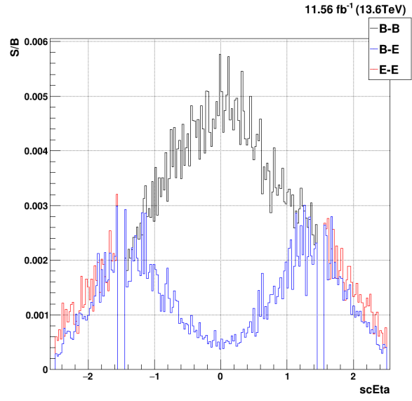
(b) Signal/Background for SA Selection
