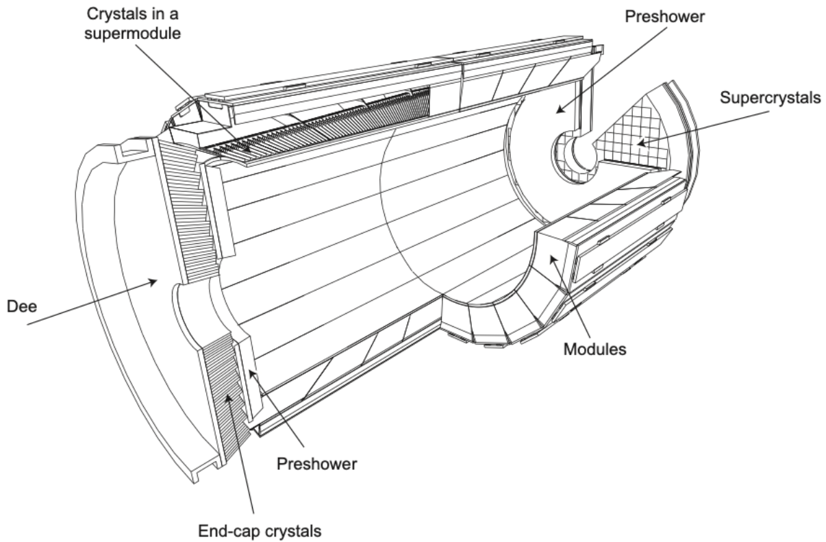
Figure 2.5. A simplified schematic of the ECal. Reproduced from [18]
