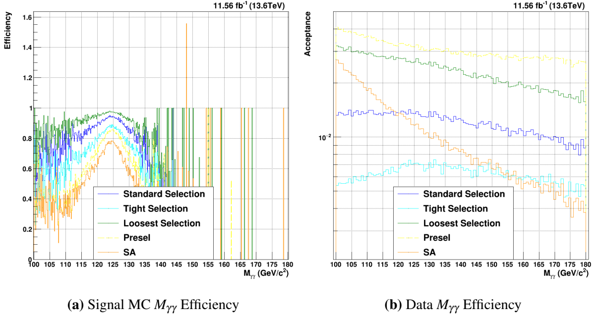
Figure 7.8. M_{\gamma\gamma} distributions for H \rightarrow \gamma\gamma events accepted by different offline selections. Three tightnesses of BDT-based selection cuts are shown in dark blue (standard), light blue (tighter), and light green (looser). The preselection is shown in yellow, while the full standard analysis cuts are shown in orange.
