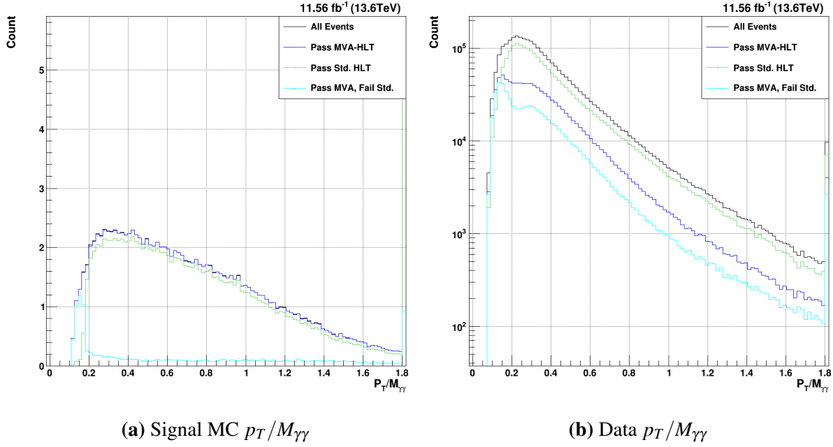
Figure 7.6. HH \rightarrow b\bar{b}\gamma\gamma p_T/M_{\gamma\gamma} distribution of events accepted by the MVA-HLT (dark blue) vs. the current diphoton sHLT (green). Events that pass the MVA-HLT but fail the sHLT can be seen in light blue.
