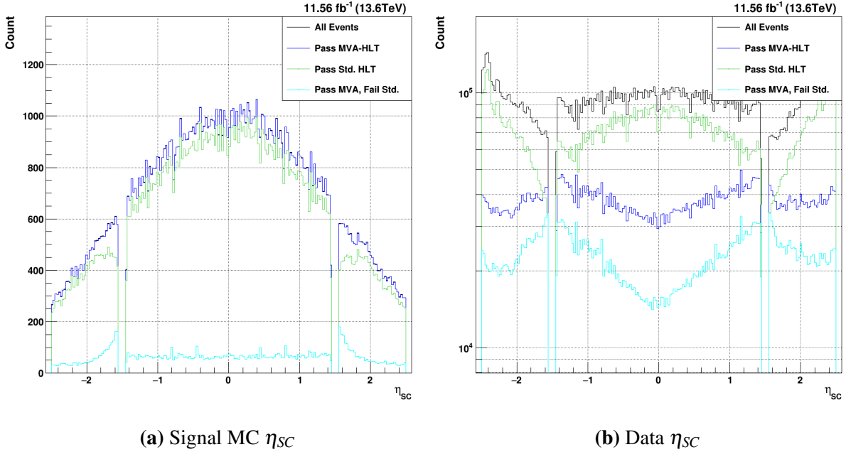
Figure 7.2. H \rightarrow \gamma\gamma \eta_{SC} distribution of events accepted by the MVA-HLT (dark blue) vs. the current diphoton sHLT (green). Events that pass the MVA-HLT but fail the sHLT can be seen in light blue.
