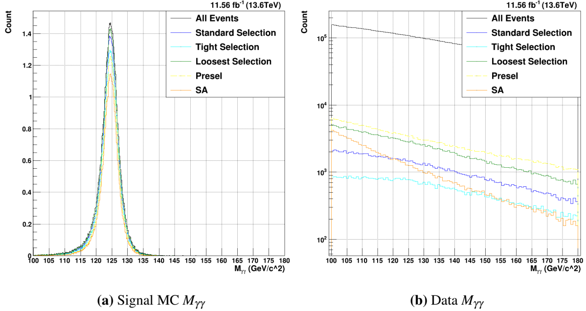
Figure 7.16. Total offline selection acceptances for HH \rightarrow b\bar{b}\gamma\gamma . Three tightnesses of BDT-based selection cuts are shown in dark blue (standard), light blue (tighter), and light green (looser). The acceptance of the preselection is shown in yellow, while the full standard analysis cuts are shown in orange.
