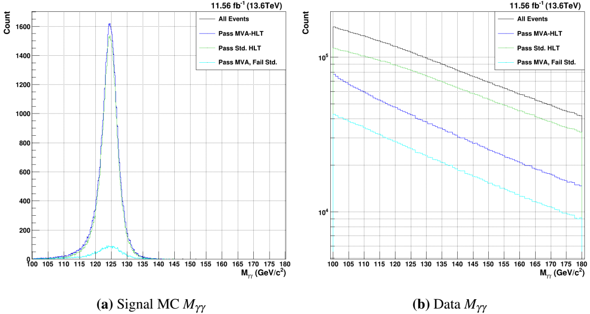
Figure 7.1. H \rightarrow \gamma\gamma M_{\gamma\gamma} distribution of events accepted by the MVA-HLT (dark blue) vs. the current diphoton sHLT (green). Events that pass the MVA-HLT but fail the sHLT can be seen in light blue.
