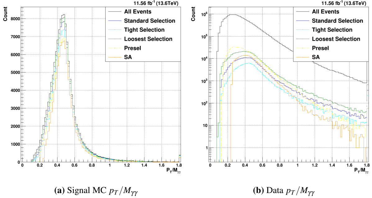
Figure 7.11. p_T/M_{\gamma\gamma} distributions for H \rightarrow \gamma\gamma events accepted by different offline selections. Three tightnesses of BDT-based selection cuts are shown in dark blue (standard), light blue (tighter), and light green (looser). The preselection is shown in yellow, while the full standard analysis cuts are shown in orange. Both the lead and sublead photons are plotted together.
