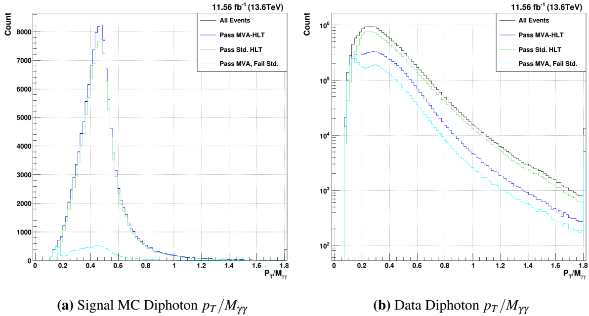
Figure 7.3. H \rightarrow \gamma\gamma p_T/M_{\gamma\gamma} distribution of events accepted by the MVA-HLT (dark blue) vs. the current diphoton sHLT (green). Events that pass the MVA-HLT but fail the sHLT can be seen in light blue.
