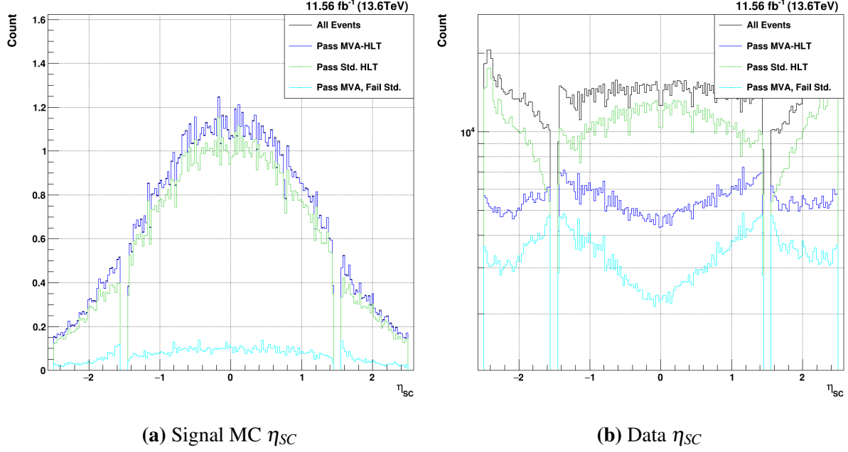
Figure 7.5. HH \rightarrow b\bar{b}\gamma\gamma \eta_{SC} distribution of events accepted by the MVA-HLT (dark blue) vs. the current diphoton sHLT (green). Events that pass the MVA-HLT but fail the sHLT can be seen in light blue.
