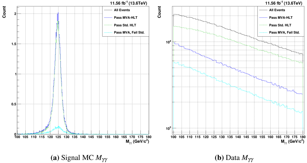
Figure 7.4. HH \rightarrow b\bar{b}\gamma\gamma M_{\gamma\gamma} distribution of events accepted by the MVA-HLT (dark blue) vs. the current diphoton sHLT (green). Events that pass the MVA-HLT but fail the sHLT can be seen in light blue.
