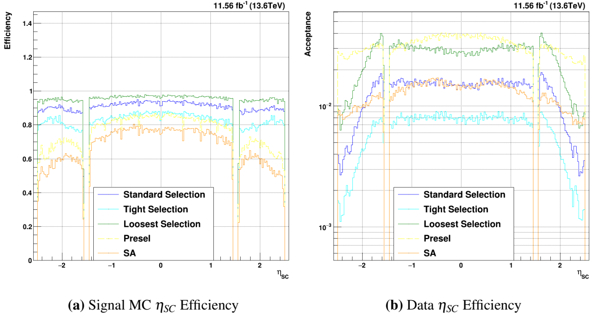
Figure 7.10. Total offline efficiency for H \rightarrow \gamma\gamma . Three tightnesses of BDT-based selection cuts are shown in dark blue (standard), light blue (tighter), and light green (looser). The acceptance of the preselection is shown in yellow, while the full standard analysis cuts are shown in orange.
