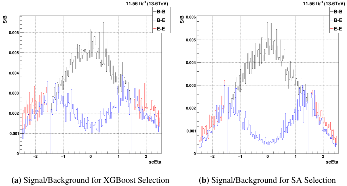
Figure 7.22. Signal/Background measurement for HH \rightarrow b\bar{b}\gamma\gamma .
