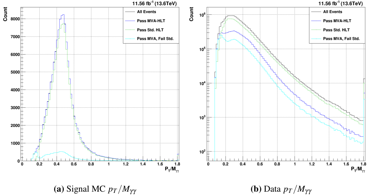
Figure 7.3. Acceptance of the MVA-HLT (dark blue) vs. the current standard diphoton HLT (green) for p_T/M_{\gamma\gamma} . Both the lead and sublead photons are plotted together. Events that pass the MVA-HLT but fail the standard HLT can be seen in light blue.
