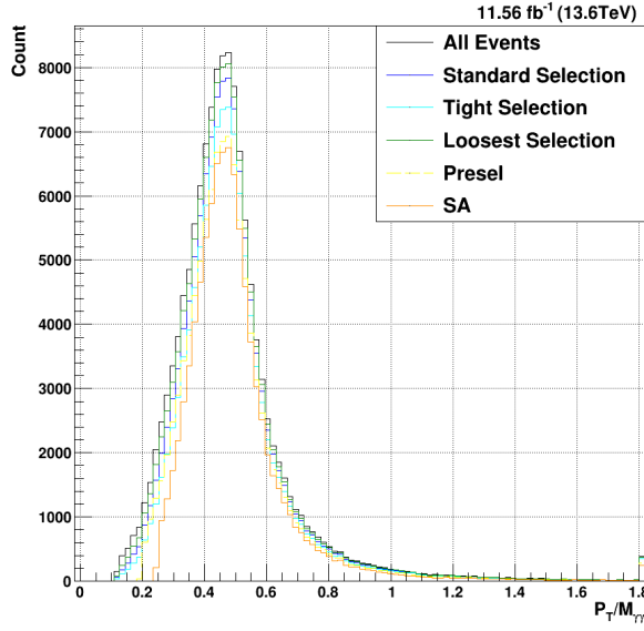
(a) Signal MC p_T/M_{\gamma\gamma}
