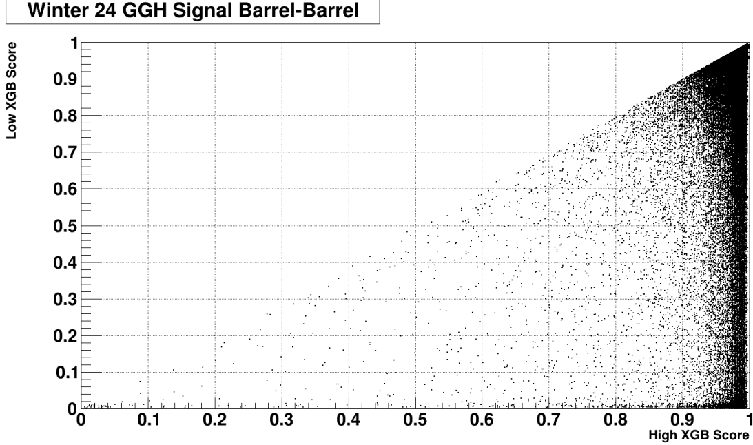
Figure 6.2. XGBoost output scores for two selected photon candidates in the Winter 2024 ggH signal MC. The higher of the two scores is plotted on the X-axis, while the lower of the two is plotted on the Y-axis.
