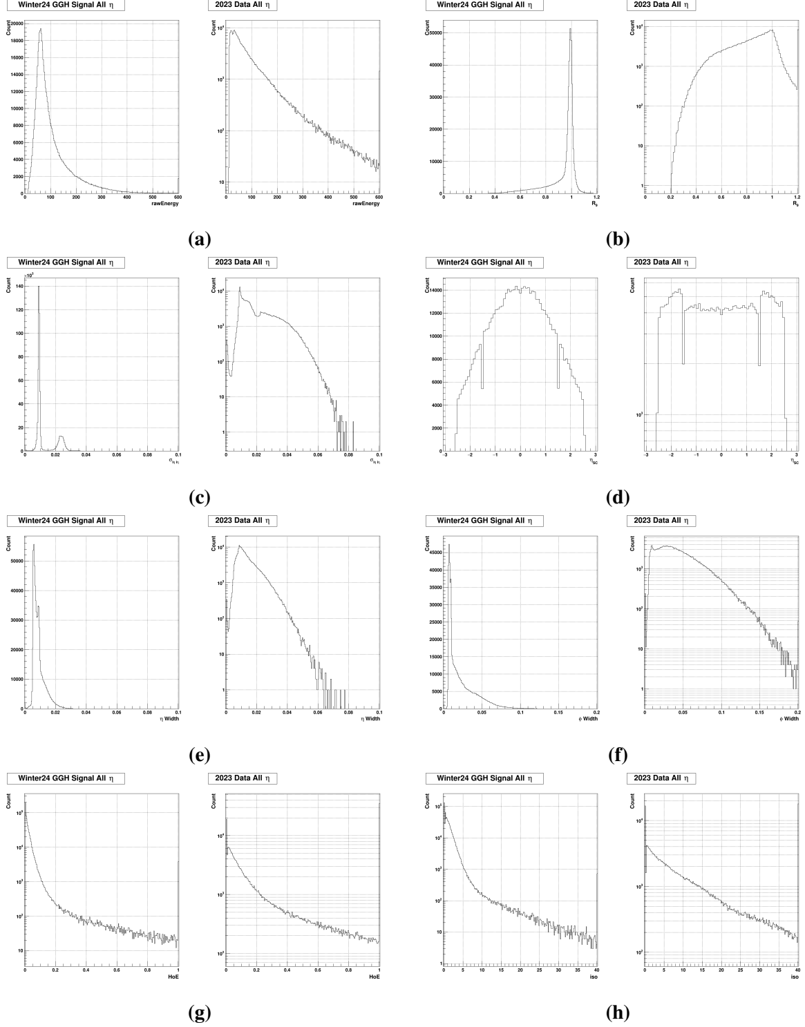
Figure 6.1. Plots of the input variables to the BDT, where the signal MC is shown on the left and the data is shown on the right
