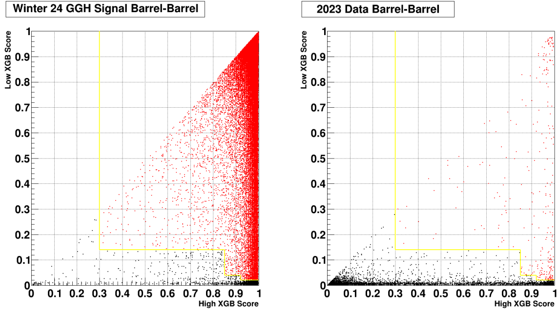
Figure 6.4. XGBoost output scores for the signal MC (left) and data (right) where both photon candidates are in the Barrel. Events accepted by the cuts are show in red, and the values of the cuts are shown by the yellow lines.
