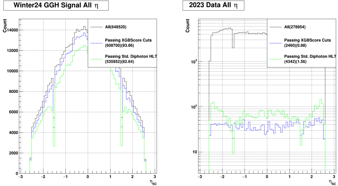
Figure 6.7. Photon \eta for the signal MC (left) and data (right). Events accepted by the MVA-HLT are shown in blue, while events accepted by the standard HLT are shown in green.
