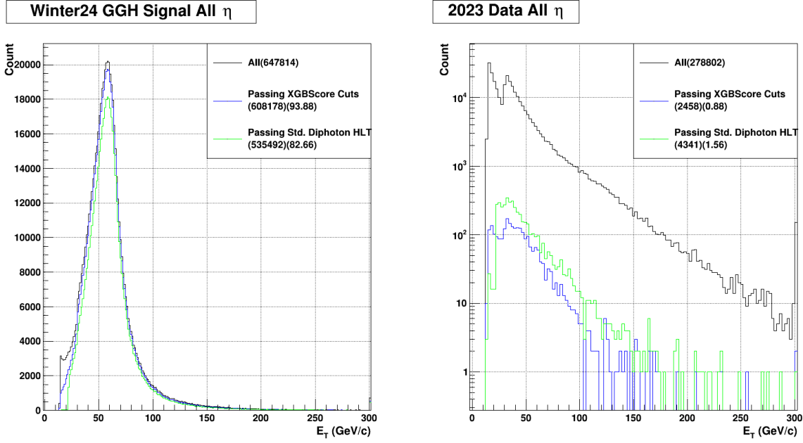
Figure 6.8. Photon E_T for the signal MC (left) and data (right). Events accepted by the MVA-HLT are shown in blue, while events accepted by the standard HLT are shown in green.
