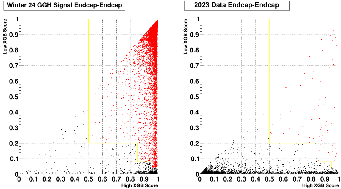
Figure 6.5. XGBoost output scores for the signal MC (left) and data (right) where both photon candidates are in the Endcap. Events accepted by the cuts are show in red, and the values of the cuts are shown by the yellow lines.
