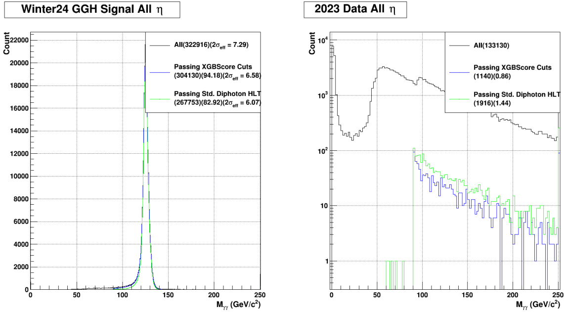
Figure 6.6. Diphoton mass for the signal MC (left) and data (right). Events accepted by the MVA-HLT are shown in blue, while events accepted by the standard HLT are shown in green.
