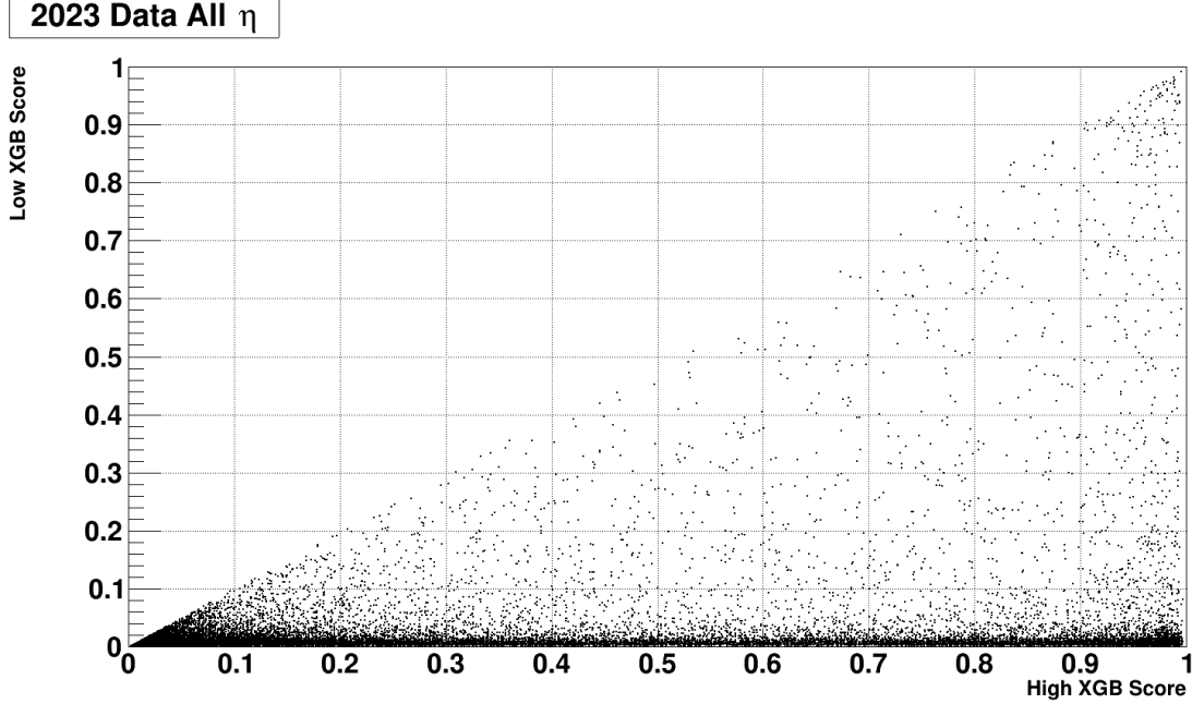
Figure 6.3. XGBoost output scores for two selected photon candidates in the 2023 Data. The higher of the two scores is plotted on the X-axis, while the lower of the two is plotted on the Y-axis.
