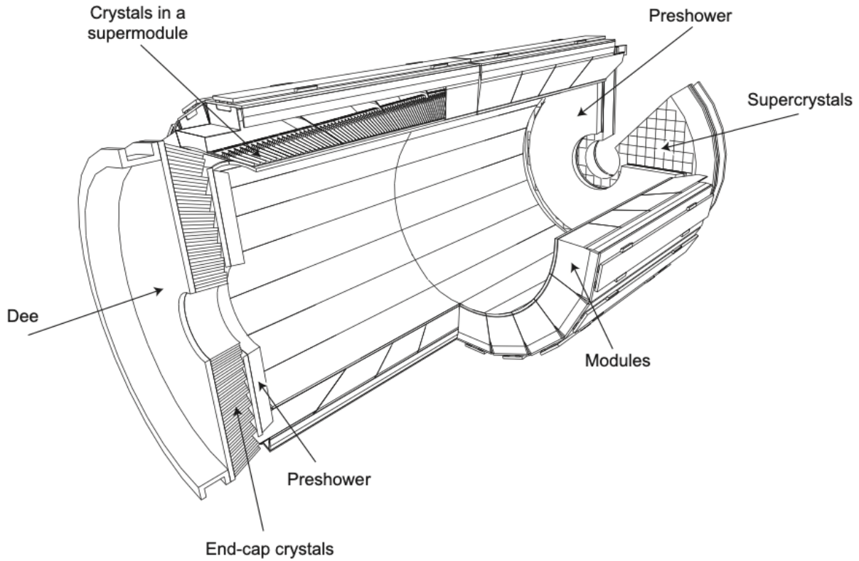
Figure 2.5. A simplified schematic of the ECal. Reproduced from [13]
