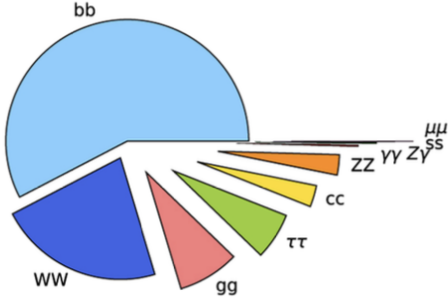
Figure 1.6. Theoretical branching fractions for a single Higgs. Reproduced from [6]
