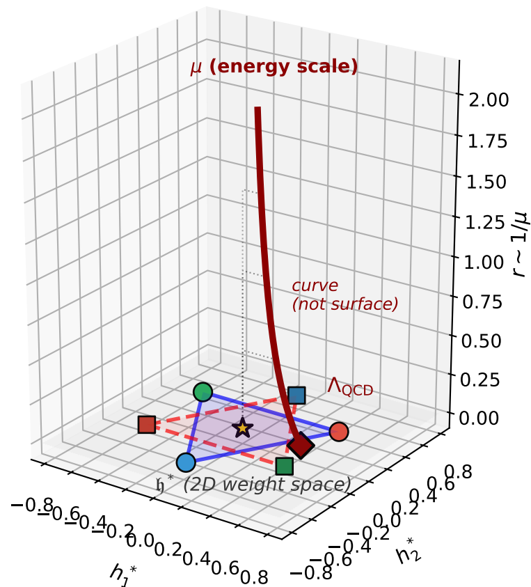
(a) RG flow adds one radial direction to color space 2 (weight) + 1 (radial) = 3
