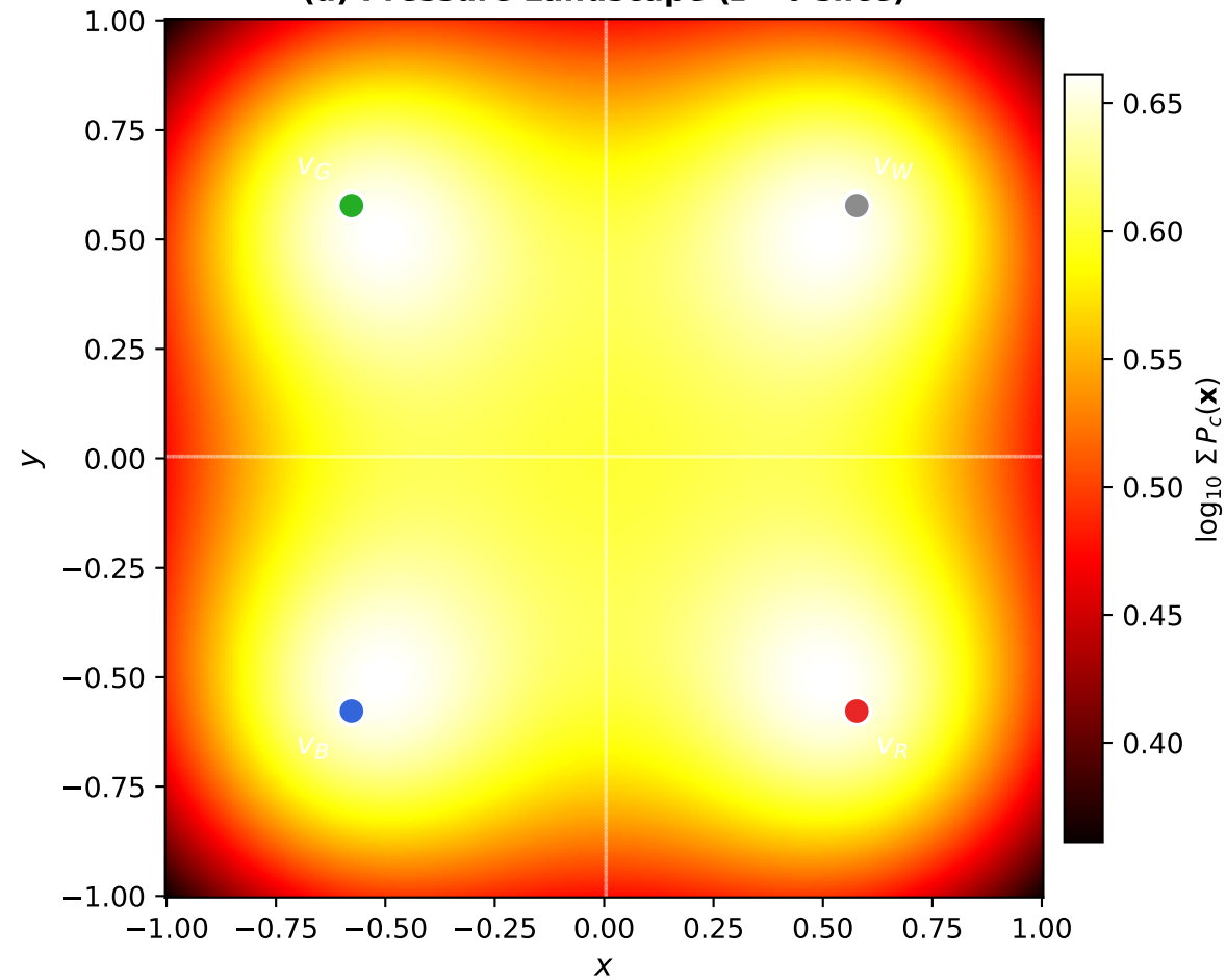
(a) Pressure Landscape ( z = 0 slice)
