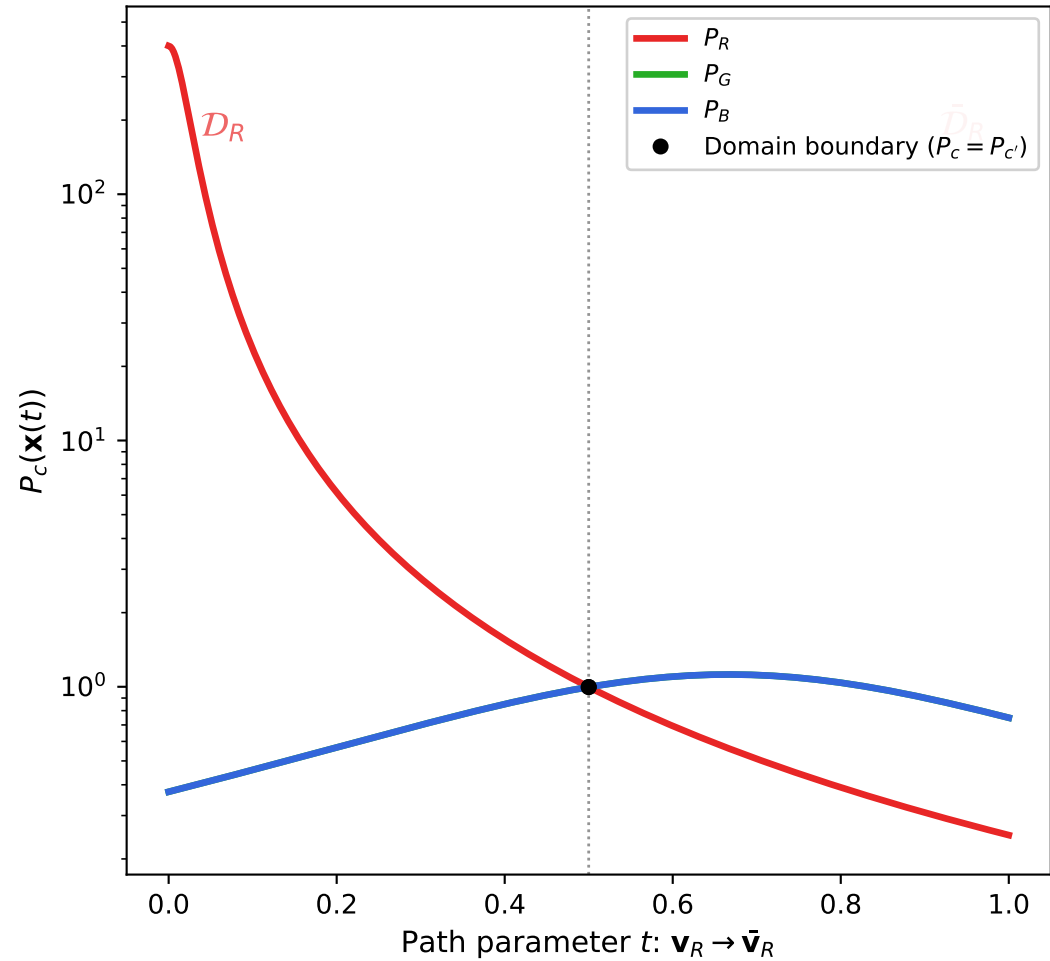
(b) Pressure Profile: V_R \rightarrow \tilde{V}_R
