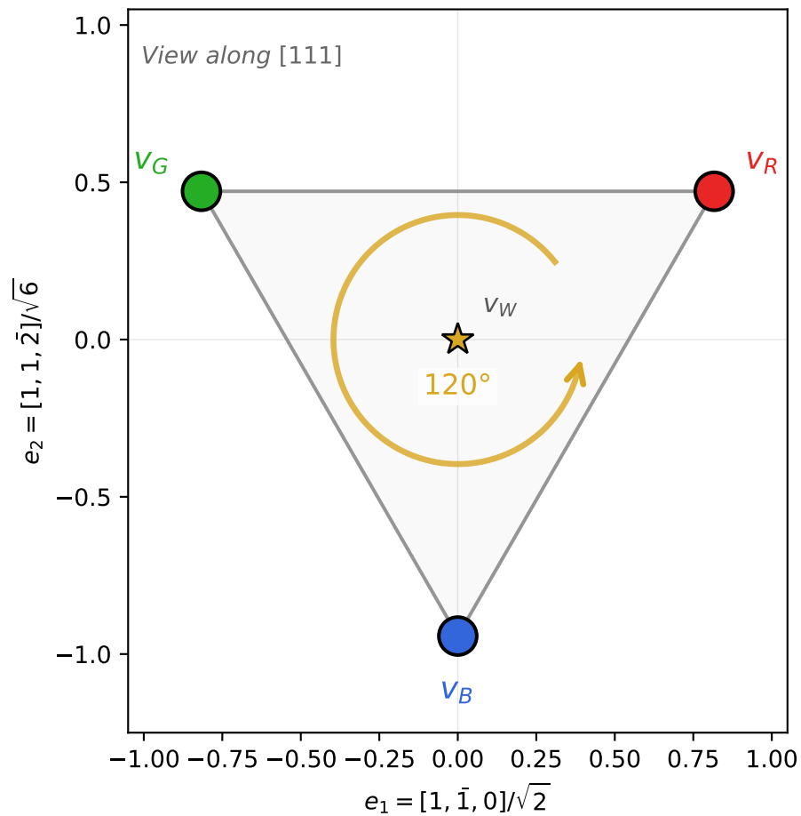
(b) \mathbb{Z}_3 Rotation: R \rightarrow G \rightarrow B
