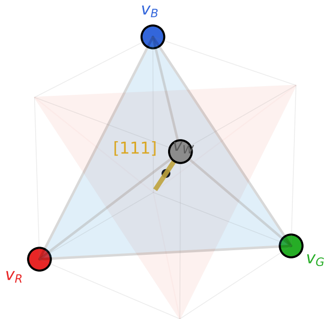
(a) Stella with \mathbb{Z}_3 Axis [111]
