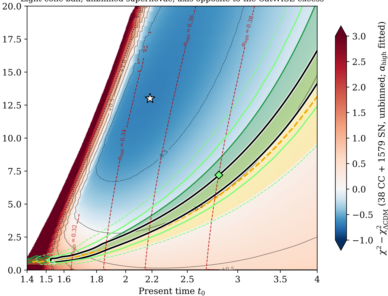
Light-cone ball, unbinned supernovae, axis opposite to the CatWISE excess
