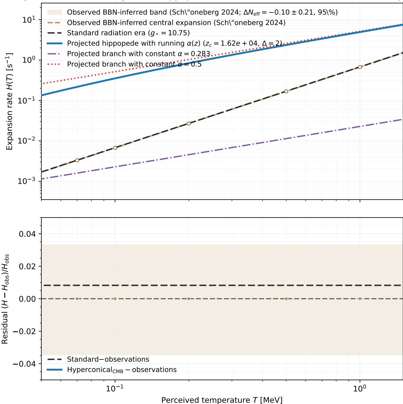
Projected thermal history of the hippopede model vs. standard and BBN-inferred expansion
