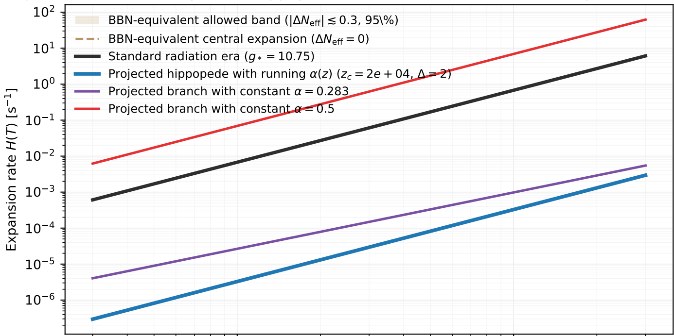
Projected thermal history of the hippopede model vs. standard and BBN-equivalent expansion
