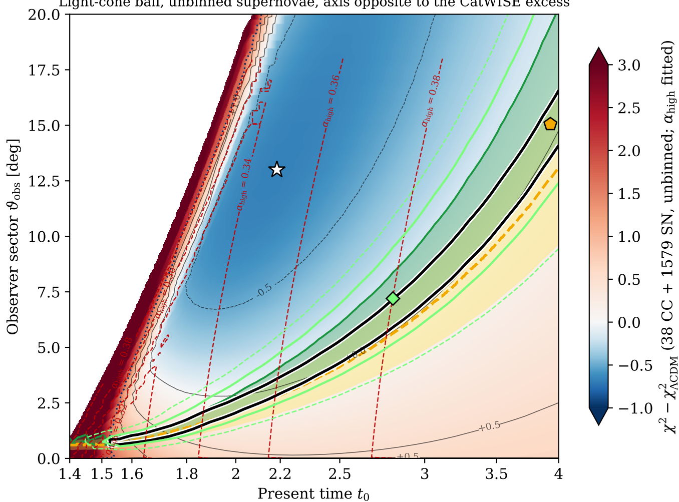
Light-cone ball, unbinned supernovae, axis opposite to the CatWISE excess
