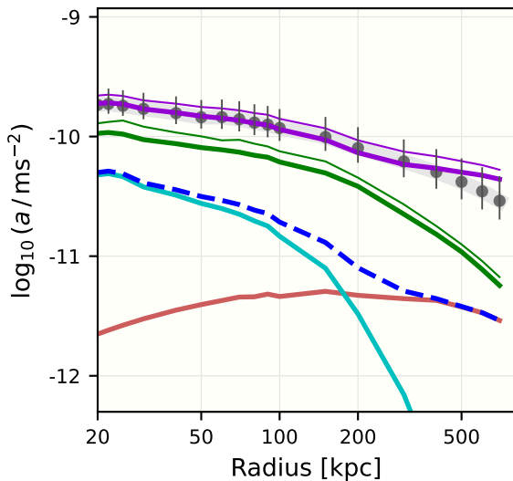
Abell-2717 cluster
