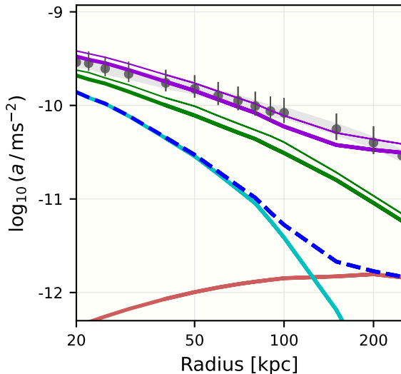
Abell-2717 cluster
