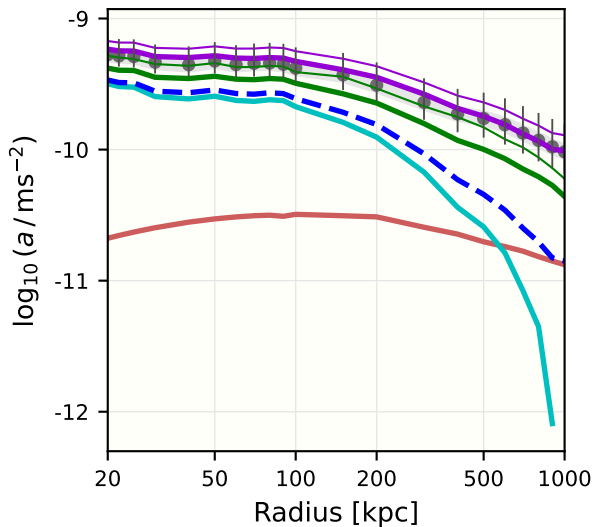
Abell-2029 cluster
