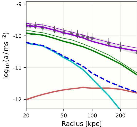
Abell-2029 cluster
