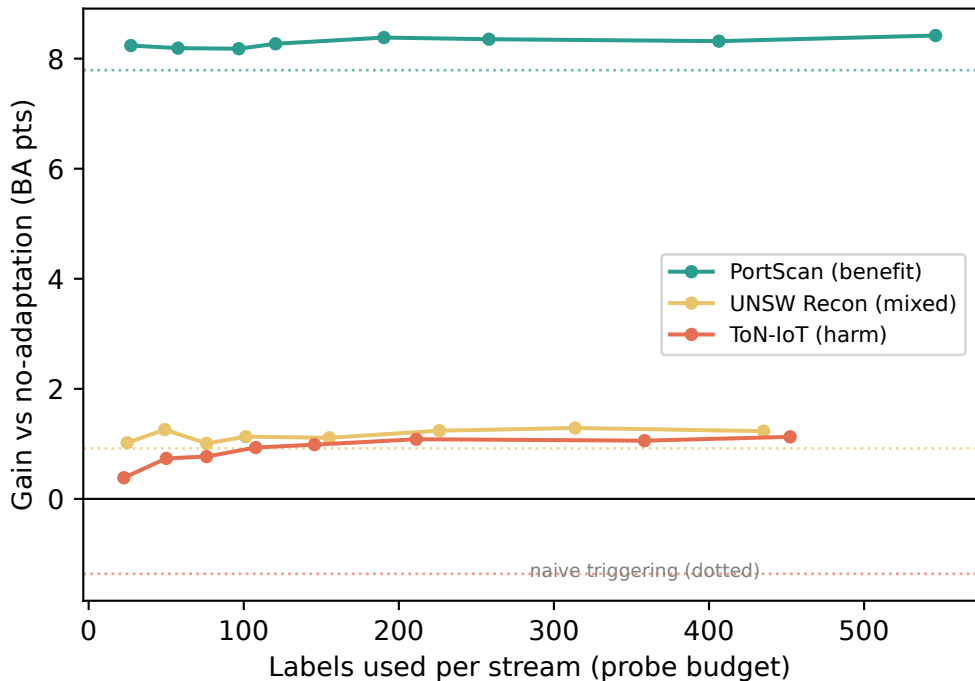
Label-efficiency frontier: a small probe suffices to avoid harm
