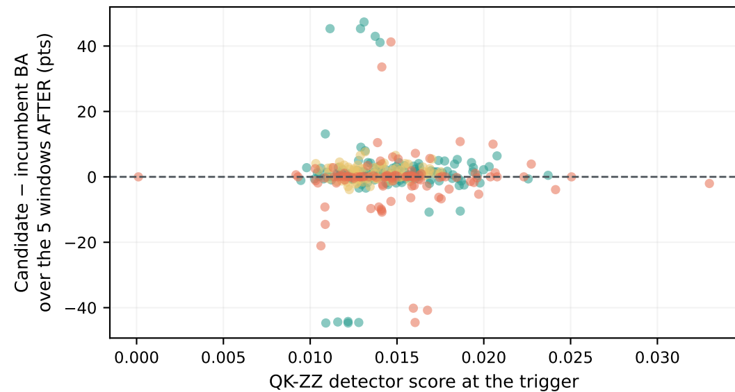
QK-ZZ (quantum) No consistent score-value association at triggers (pooled r = +0.01 )
