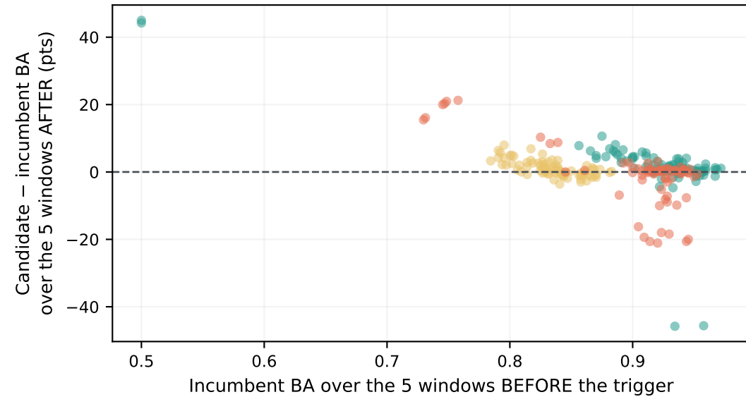
KS-max (classical) Incumbent health predicts the value of committing (pooled r = -0.57 )
