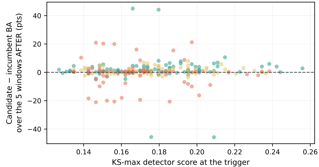
KS-max (classical) No consistent score-value association at triggers (pooled r = +0.02 )
