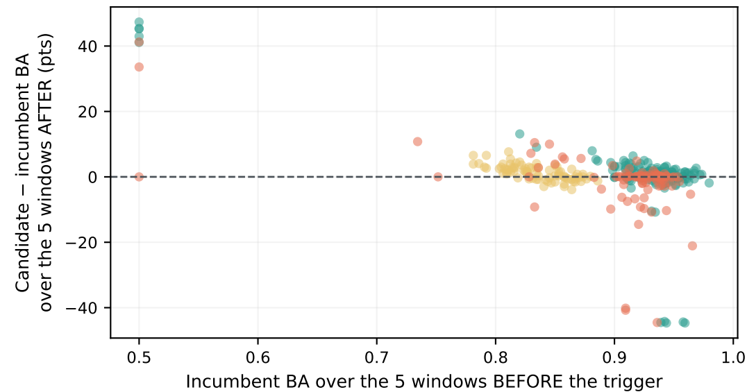
QK-ZZ (quantum) Incumbent health predicts the value of committing (pooled r = -0.59 )
