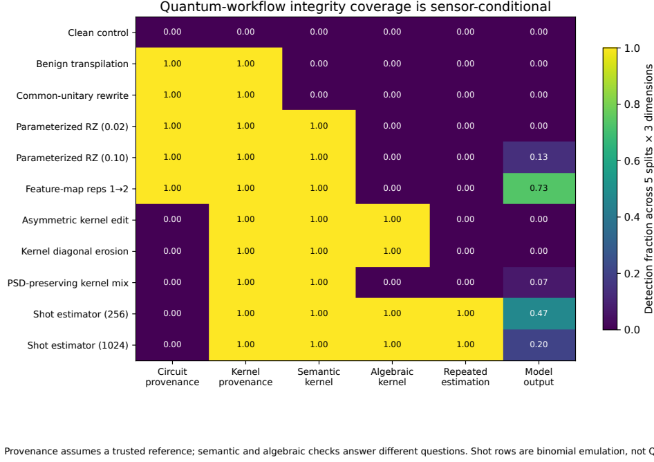
Fig. 3. Sensor response across clean and semantics-preserving controls, circuit mutations, kernel corruptions and finite-shot emulators over 165 simulator cells. Coverage is conditional on the evidence exposed to each sensor; output invariance does not imply workflow integrity.
