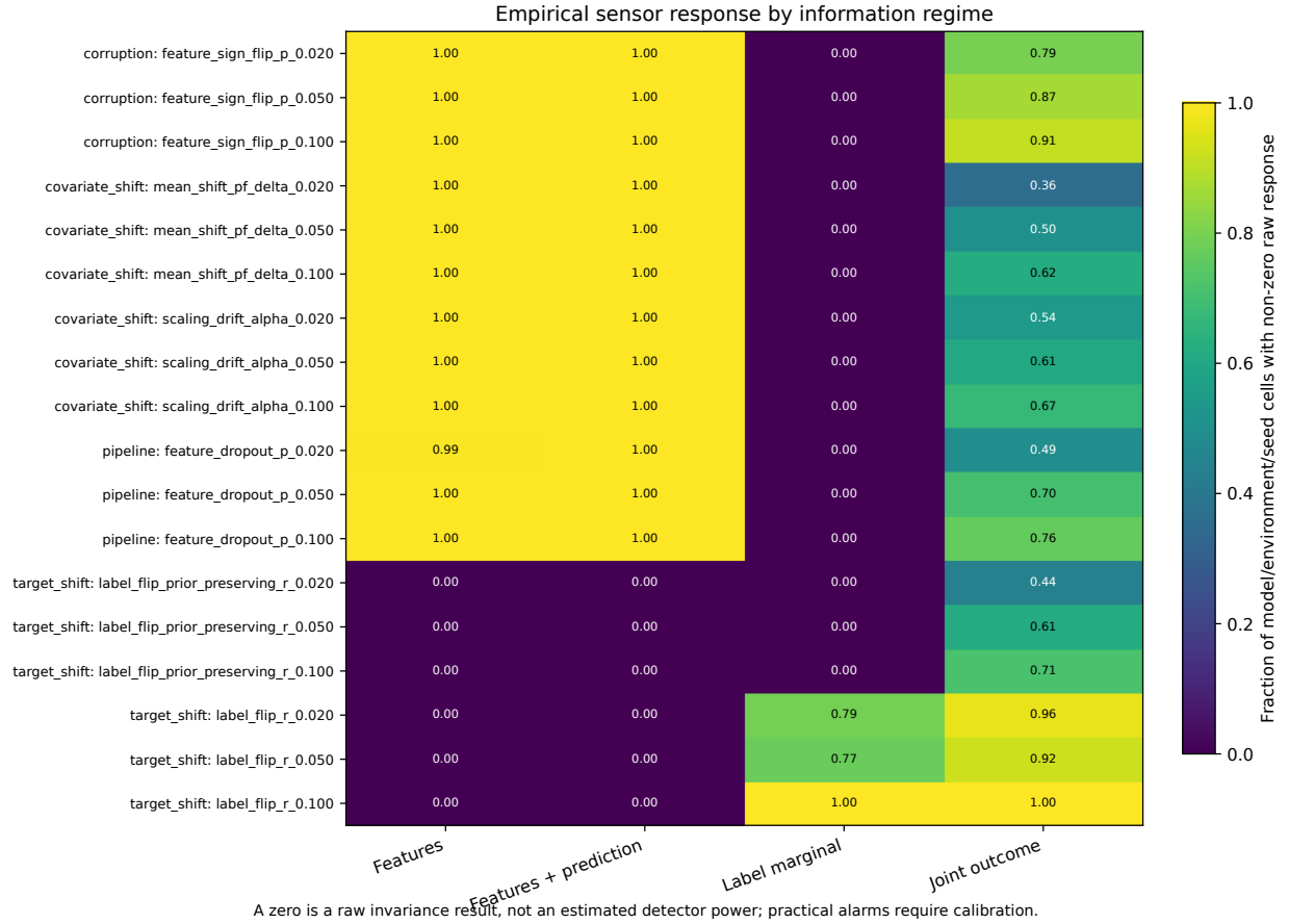
Fig. 4. Raw sensor response by information regime in the frozen expansion. Fractions are over model/environment/seed cells; zero denotes raw invariance, not estimated detector power.
