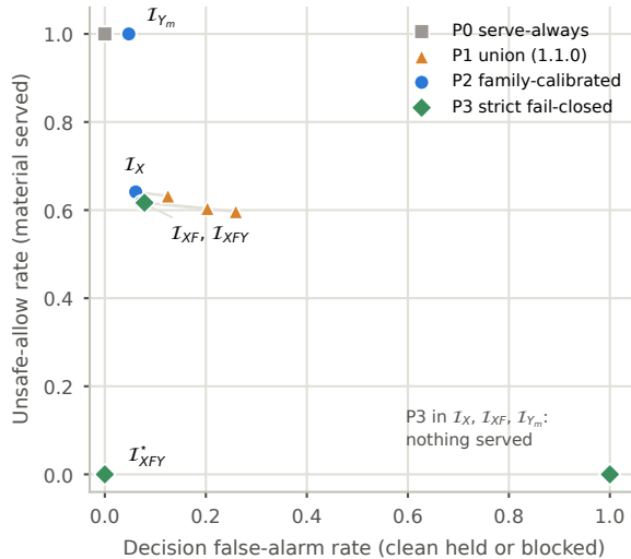
(a) Per-sensor \alpha = 0.05 does not calibrate the decision (b) Unsafe allow versus false hold, |\Delta_R| > 0
