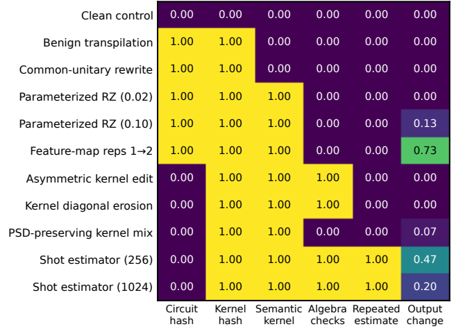
Fig. 1. Response fraction of each quantum-branch sensor over the 15 cells (five splits, three dimensions) of every condition of the 165-design-cell simulator gate (0 = no cell responds, 1 = every cell); the values of Table 7. Circuit and kernel hashes are the provenance sensors; the anchored-kernel column compares against \Phi(C_0) , serving as a semantic probe for circuit-side rows and an observed-kernel reference for post-processing rows in this ideal gate. Coverage is conditional on the evidence exposed to each sensor; output invariance does not imply workflow integrity, and the shot rows are binomial emulation, not QPU runs.
