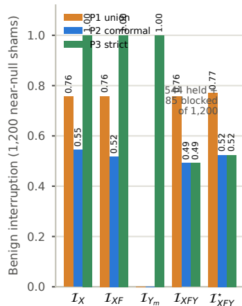
(c) Cost on benign in-place variation
