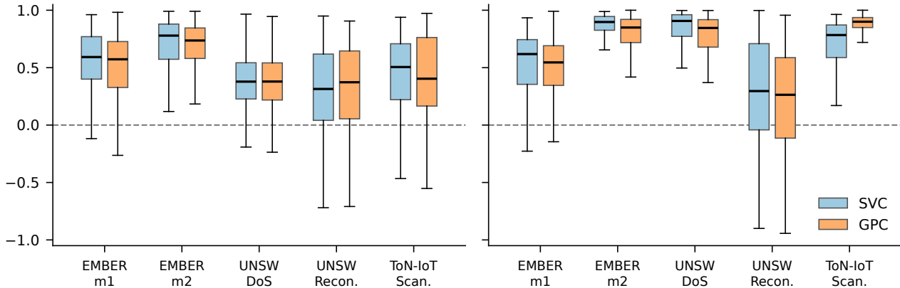
Cross-fit \rho(KTA_A, acc_B) , disjoint halves
