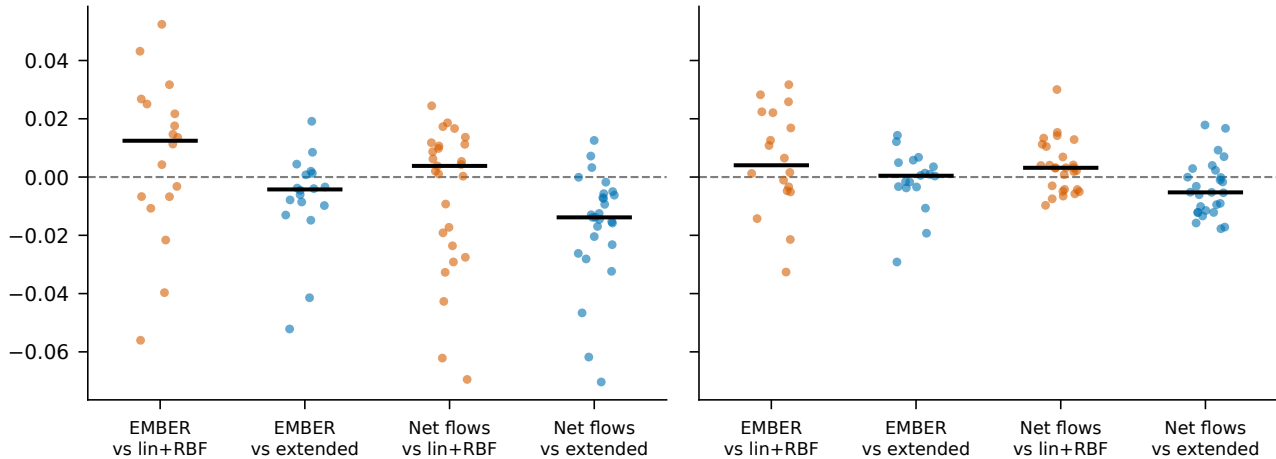
SVC
