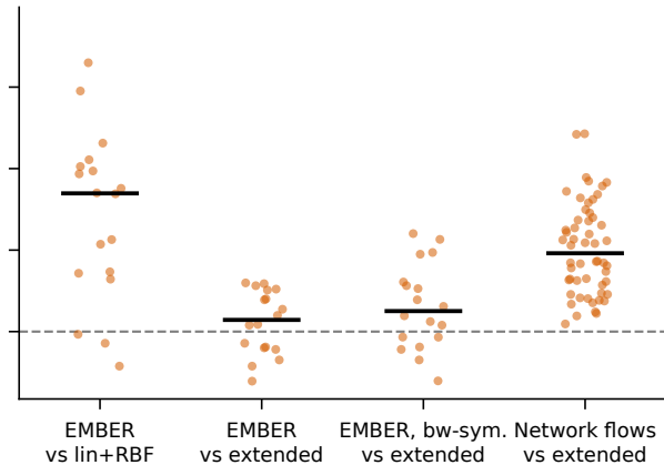
GP classifier
