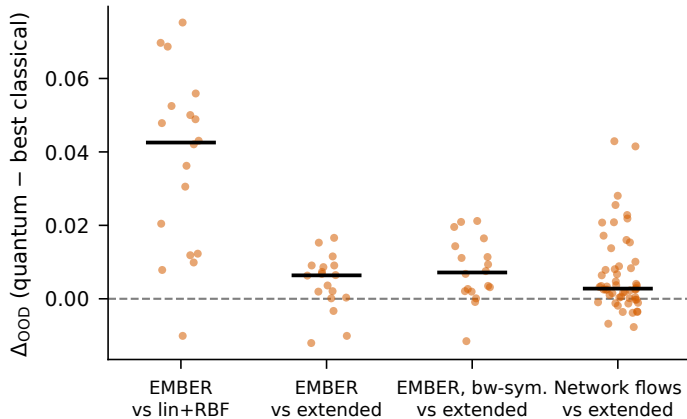
SVC
