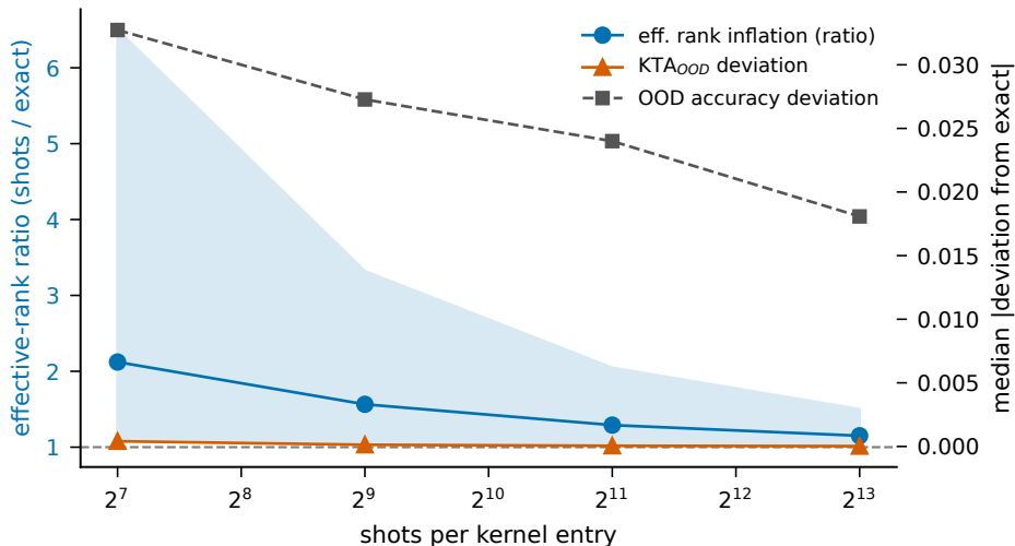
Finite shots inflate effective rank; KTA and accuracy survive
