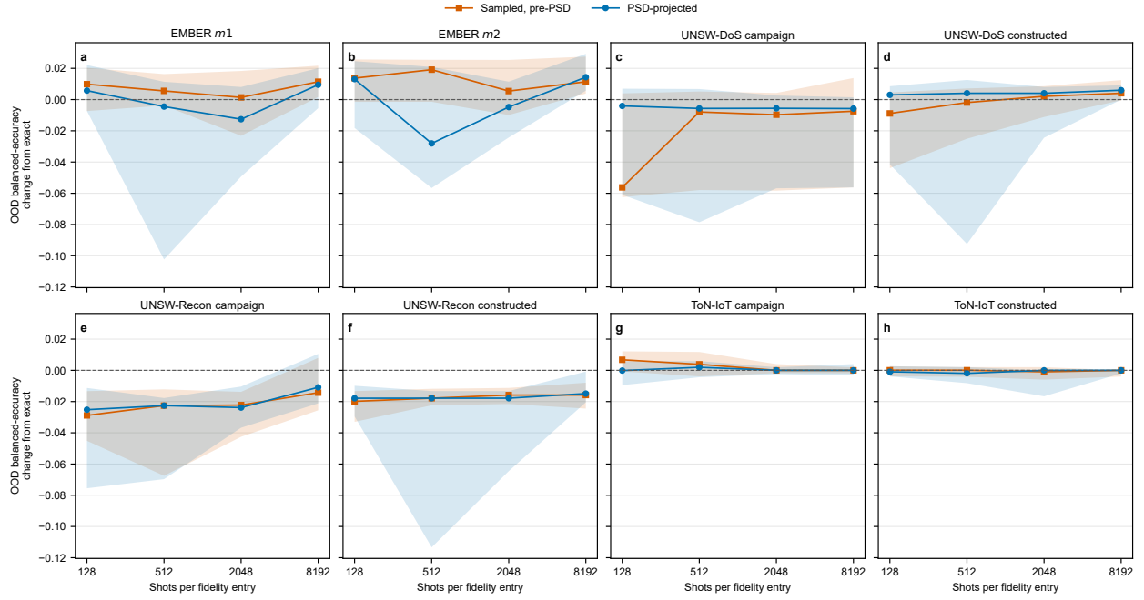
Supplementary Figure 2: Repeated finite-shot OOD change from the exact fixed-configuration end-point. Panels show one fixed scenario-group Gram matrix. Lines are medians over 30 independently seeded measurement replicates and shaded regions are central 95% Monte Carlo intervals ( n = 30 ) conditional on that matrix. Orange squares use the sampled indefinite matrix; blue circles use its PSD projection. The model includes fidelity sampling only, not device noise.
