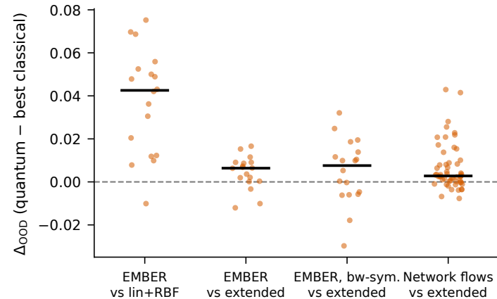
SVC
