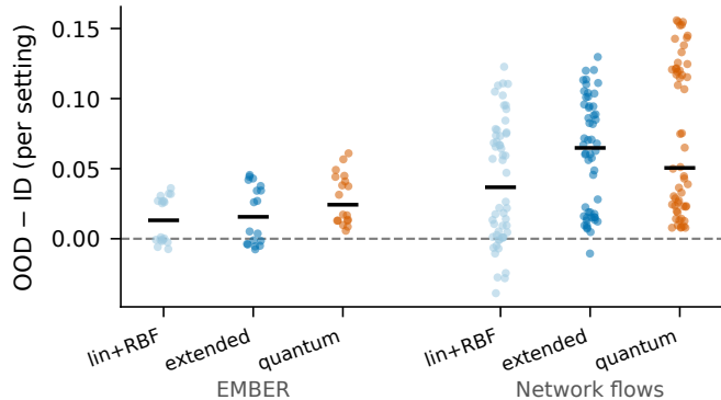
Predictive entropy rises under shift
