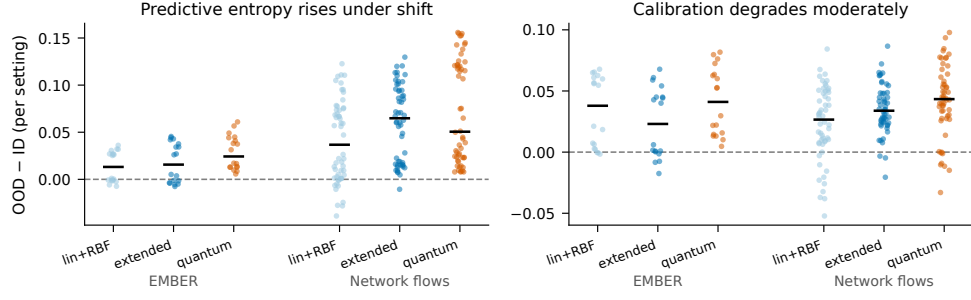
Fig. 5 Predictive uncertainty under shift. Per-setting ID-to-OOD change in mean predictive entropy (left) and expected calibration error (right) for the Best-by-OOD configuration of each family under the GP classifier; black bars mark medians.
