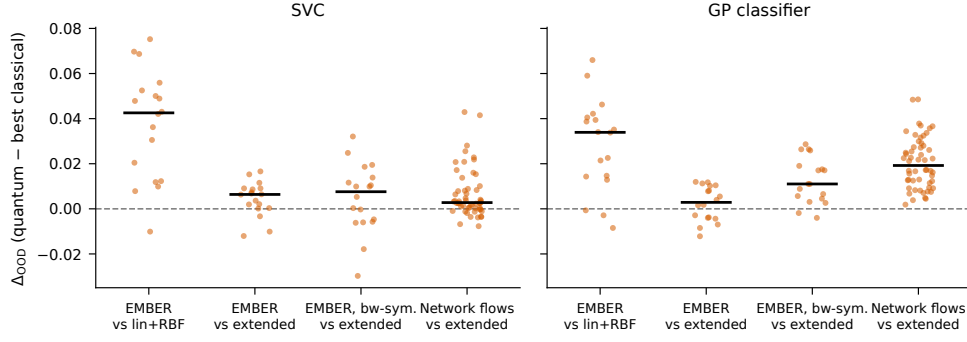
Fig. 1 The four movements of the study. Per-setting Best-by-OOO deltas (quantum minus best classical, mean over 15 runs), for SVC (left) and the GP classifier (right); black bars mark medians. Against linear+RBF the quantum advantage is large and nearly uniform; the extended classical family collapses it on EMBER; symmetric bandwidth tuning partially restores it; on network flows (54 settings, including natural drift) it persists against the extended family, uniformly so under the GP classifier.
