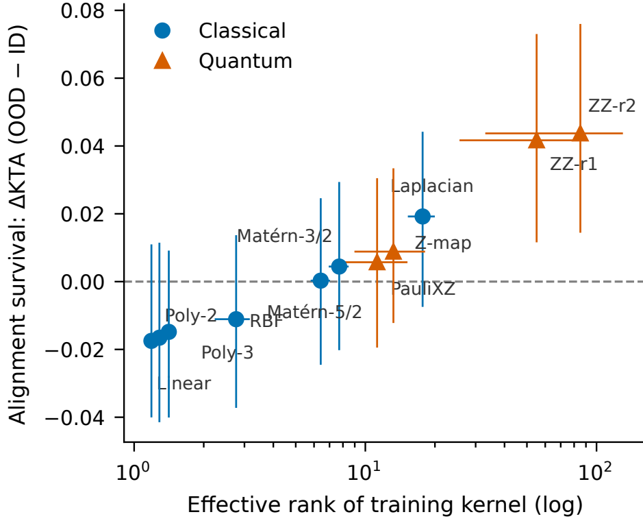
Fig. 3 Effective rank versus alignment survival across both kernel families. Markers are means over the 18 EMBER settings and 5 dimensions; bars span interquartile ranges. The relationship is monotone across both families: the classical kernels that retain alignment under shift are exactly the heavy-tailed ones, and the fidelity maps occupy the high-rank end of the same continuum.
