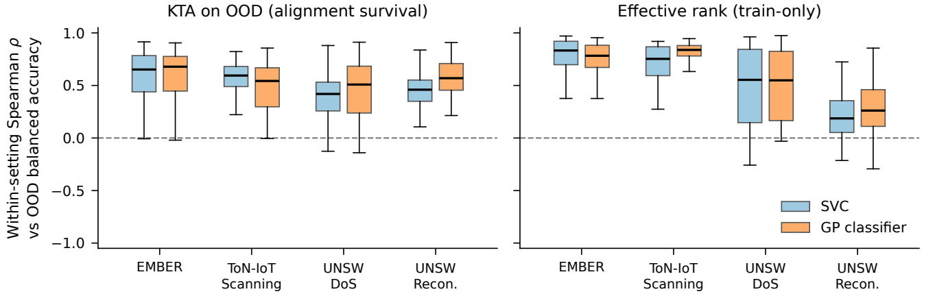
Fig. 2. The mechanism is a cross-dataset regularity. Distribution of within-setting Spearman correlations between each geometry descriptor and OOD balanced accuracy, over all setting-seed units, per dataset and classifier. Alignment survival (left) is positively correlated with OOD accuracy essentially everywhere; effective rank (right) is strong on EMBER and ToN-IoT and weaker, though still predominantly positive, on the UNSW scenarios.
