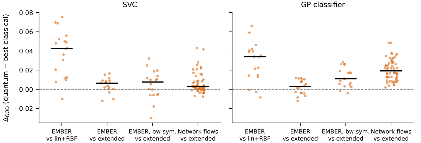
Fig. 1. Per-setting Best-by-OOD deltas (quantum minus best classical, mean over 15 runs) across the four movements of the study, for SVC (left) and the GP classifier (right). Black bars mark medians. Against linear+RBF the quantum advantage is large and nearly uniform; the extended classical family collapses it on EMBER; symmetric bandwidth tuning partially restores it; on network flows (54 settings, including natural drift) it persists against the extended family, uniformly so under the GP classifier.
