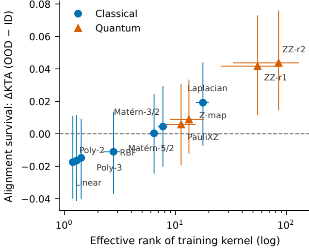
Fig. 3. Effective rank versus alignment survival for every kernel in the study (means over the 18 EMBER settings and 5 dimensions; bars span interquartile ranges). The relationship is monotone across both families: the classical kernels that retain alignment under shift are exactly the heavy-tailed ones, and the fidelity maps occupy the high-rank end of the same continuum.
