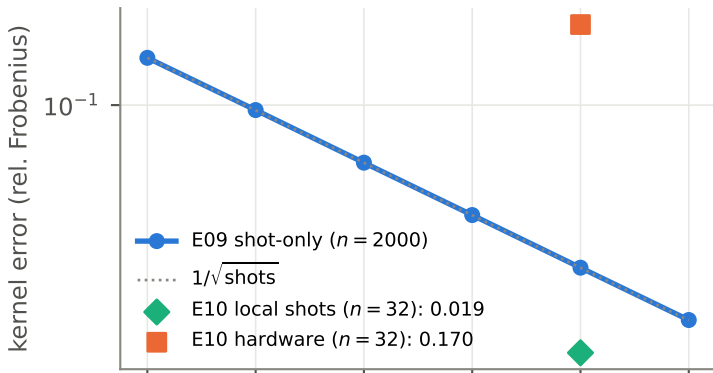
Kernel error (E09 and local E10 scales differ)
