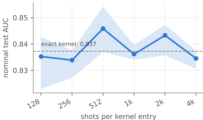
E09 downstream AUC ( n = 2000 )
