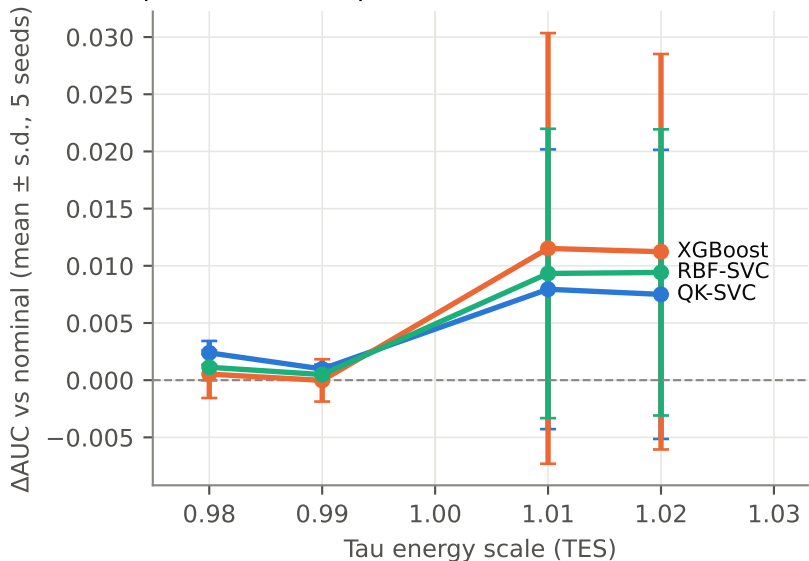
Replicated TES response (matched 2000-event models)
