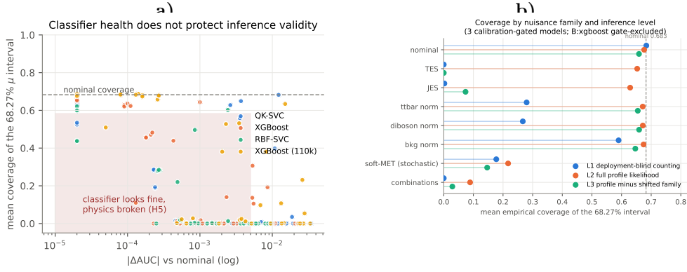
Fig. 7 Physics decoupling; (a) counting, (b) inference levels. (a) Coverage vs |\Delta AUC for the deployment-blind counting estimator: validity collapses at flat AUC. (b) Coverage by nuisance family at L1/L2/L3 under shared simulation: the fixed-template profile recovers most representable scale/normalization cells and fails where the morph cannot represent the shift (soft-MET, combinations); one JES cell is a disclosed exception. Independent-MC results separately show that auxiliary-template quality is a second validity condition.
