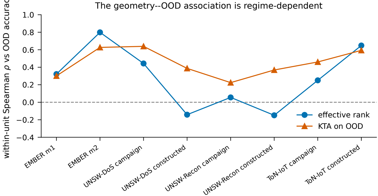
Supplementary Figure 5: The geometry--OOD association is regime-dependent. Points are median within-unit Spearman correlations between each descriptor and OOD balanced accuracy for SVC. Effective rank is strong in some regimes and weak or negative in others; OOD alignment is more consistently positive but reuses the target labels. These descriptive associations do not identify a causal mechanism.
