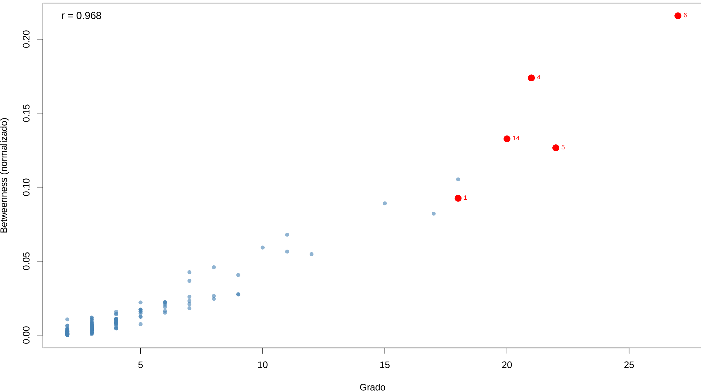
Grado vs. Betweenness – Red BA (n=200)
