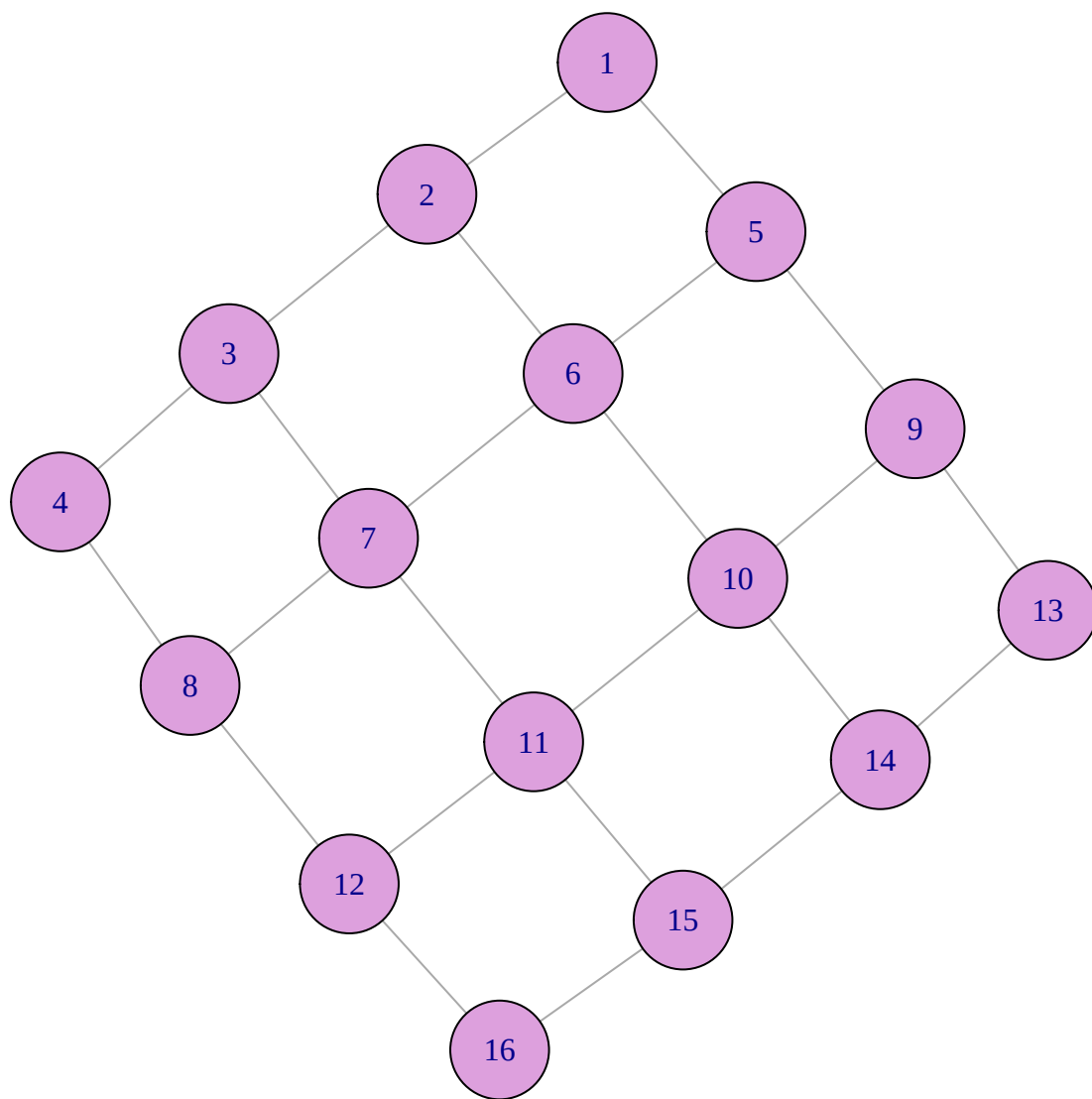
Figure 1.11: Red tipo rejilla (lattice) de 4×4
