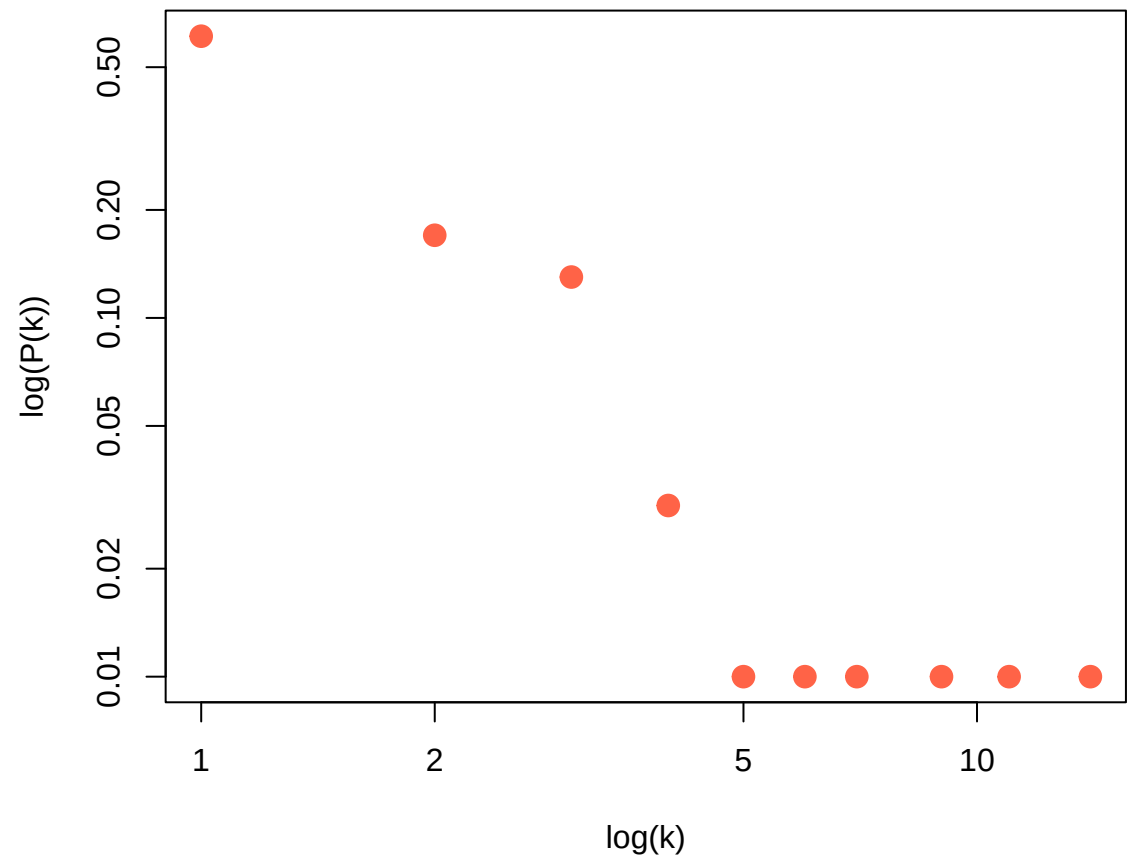
Log-log - Red BA
