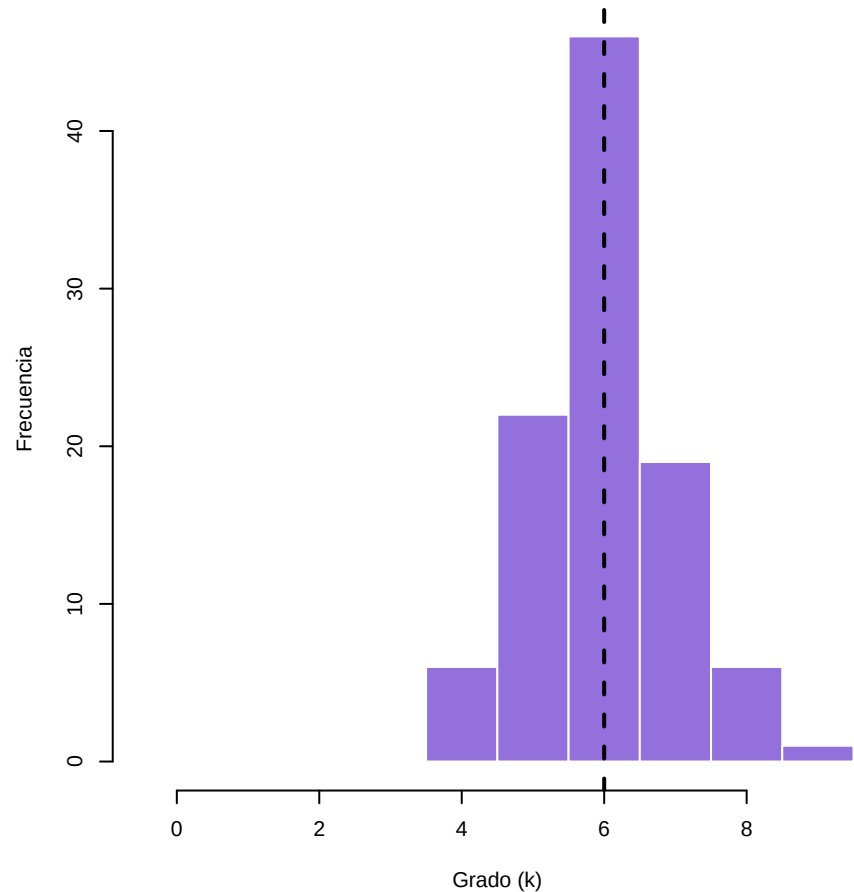
Small-World (WS)
