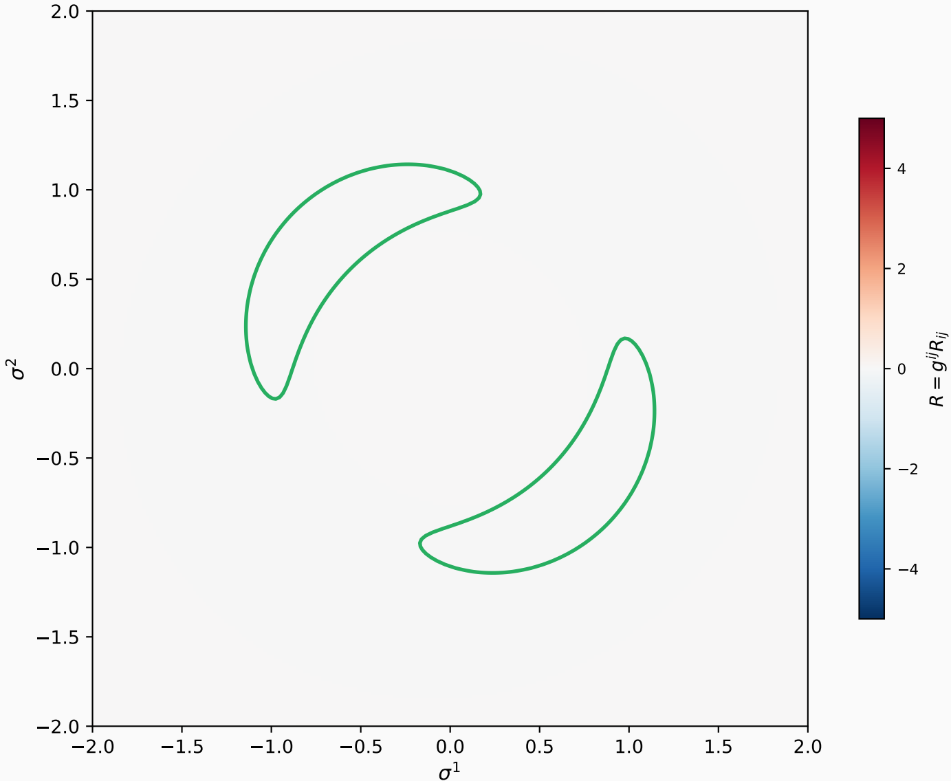
(c) Scalar Curvature R(\sigma)
