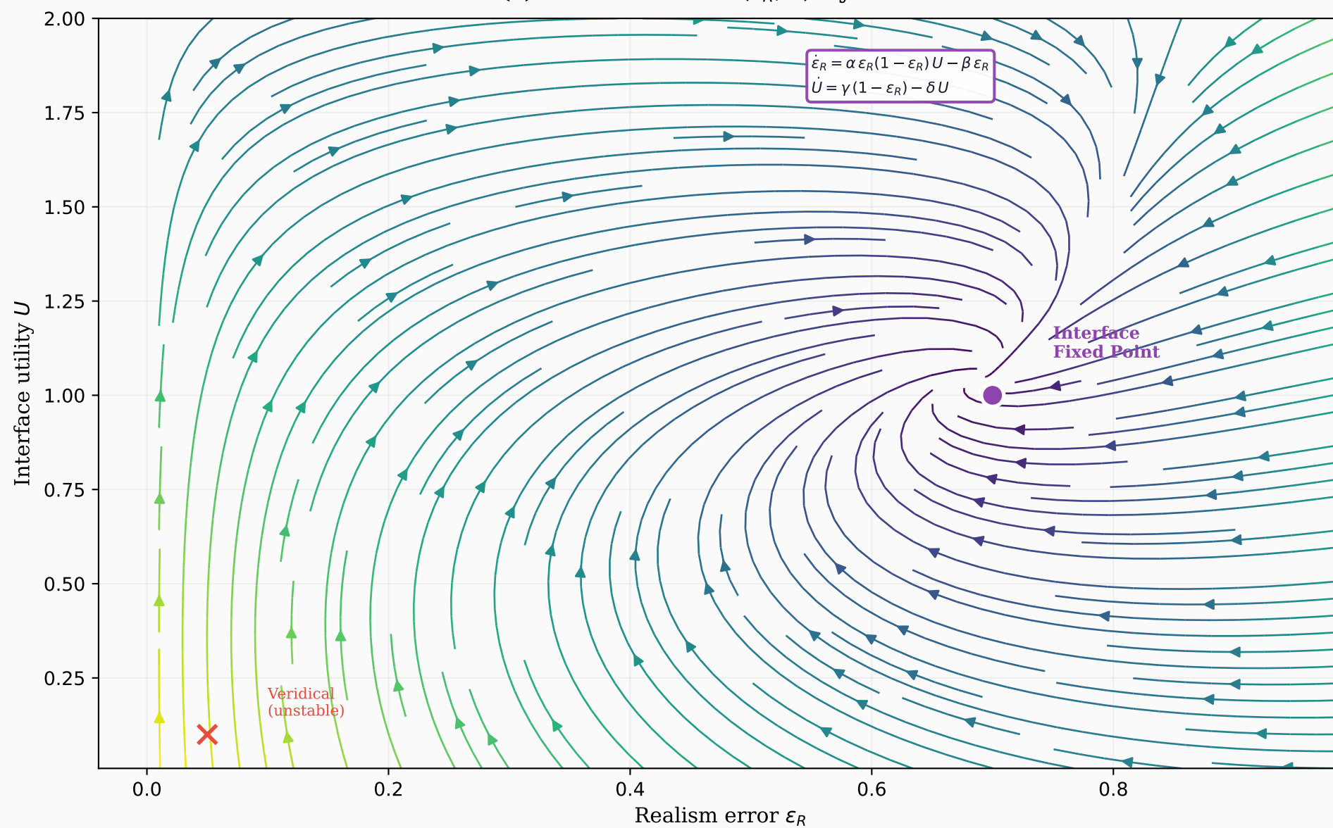
(c) Phase Portrait: (\epsilon_R, U) Dynamics
