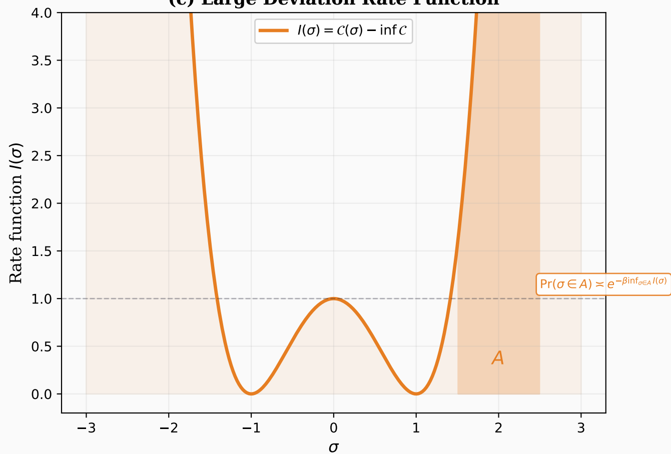
(c) Large Deviation Rate Function
