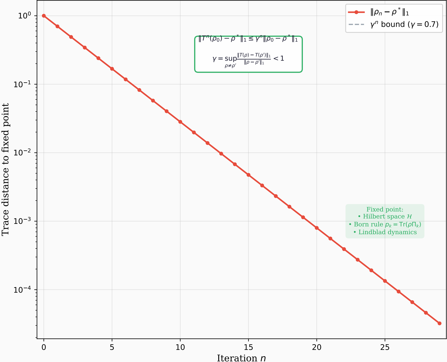
(b) Convergence: T^n(\rho_0) \rightarrow \rho^*
