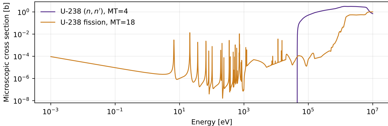
U-238 evaluated neutron cross sections
