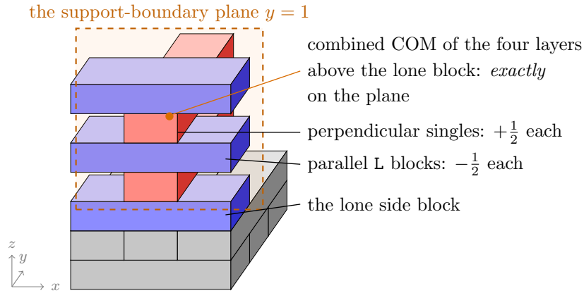
Figure 2: The knife-edge configuration. The lone side block's support ends at the plane y = 1 ; each perpendicular layer's unavoidable +\frac{1}{2} exactly cancels each parallel layer's best possible -\frac{1}{2} , parking the centre of mass of everything above precisely on the boundary.
